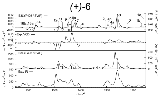
Figure 10: Comparison of experimental and calculated (B3LYP-D3/SV(P)) gas phase, frequencies scaled by 0.9614) IR and VCD spectra of (+)- 6 . Numbered VCD vibrations correspond to those analyzed in detail (Table 3, Figure 12).
