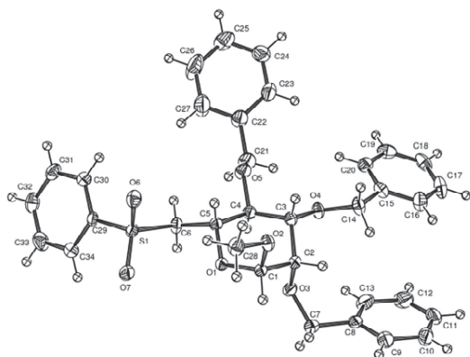
Figure 2. ORTEP drawing of 5 .
