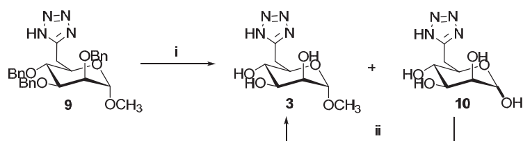
Scheme 2. Two-steps synthesis of 3 , by deprotection of hydroxyl groups of 9 followed by methylation of the obtained reaction mixture. Reactions, conditions and yields: (i) \text{BCl}_3 , \text{Cl}_2\text{H}_2 ; 3 min at -78^\circ\text{C} ; (ii) \text{SOCl}_2/\text{MeOH} , 3h at r.t.; 36% over the two steps (i) and (ii).
