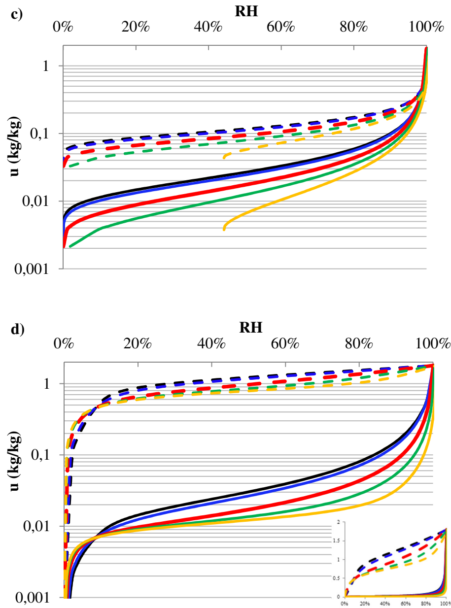
Figure 6 Main adsorption and desorption isotherms at different temperatures: a) PB equation associated with VG equation, b) PB equation associated with GAB equation, c) ThD model associated with VG equation and d) ThD model associated with GAB equation
