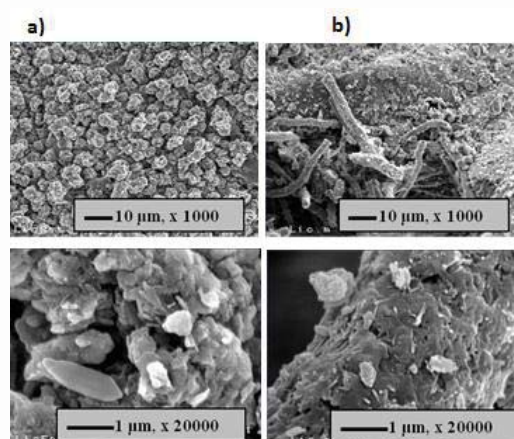
Figure 1. SEM on P. furfuracea after grinding. a) Raw sample b) Pieces obtained after grinding in a blender ( medulla pieces )
