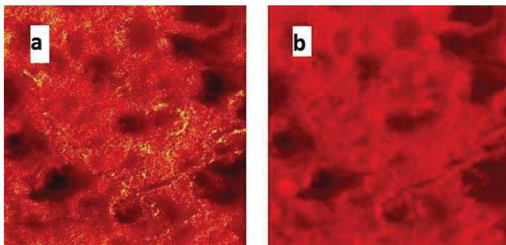
Figure 3. TOF-SIMS images (500 \mu\text{m} x 500 \mu\text{m} ) of P. furfuracea thallus a) surface b) sub-surface (removal of ca 5.5 \mu\text{m} surface material) after cluster argon beam cleaning of the surface. The yellow color indicates the atranorin (M+H) + content and red corresponds to the total ions acquired.
