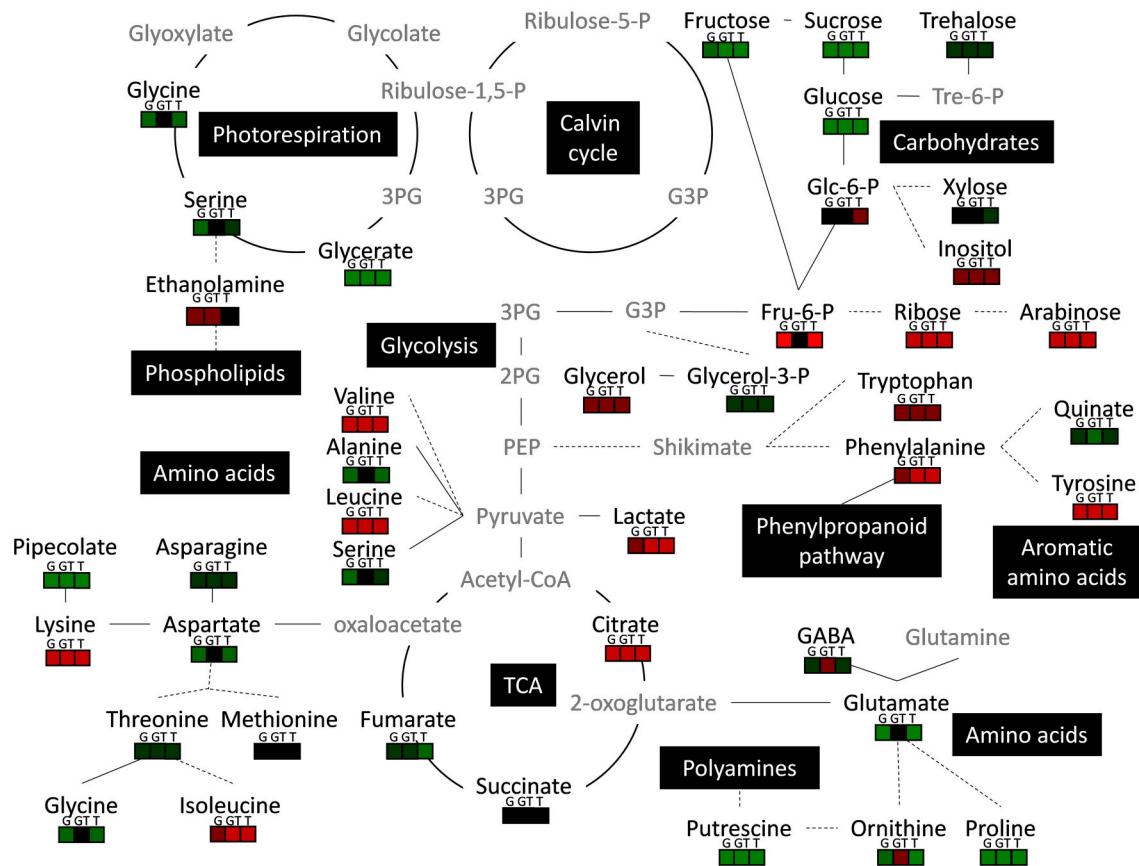
FIGURE 6 | Metabolic integration of low-intensity xenobiotic stress in L. perenne . Black names represent quantified metabolite and gray names represent non-quantified metabolites. 2PG, 2-Phosphoglycerate; 3PG, 3-Phosphoglycerate; APS, adenosine 5'-phosphosulfate; G3P, glyceraldehyde-3-phosphate; PEP, Phosphoenolpyruvate; SAMDC, S-adenosylmethionine decarboxylase; Spd, spermidine; Spm, spermine. The red or green colors respectively indicate increase or decrease of metabolite levels in the presence of glyphosate (G), tebuconazole (T) and a combination of glyphosate and tebuconazole (GT) compared to the control condition. Solid line indicate direct relation between metabolites, and dotted line show indirect reaction.
