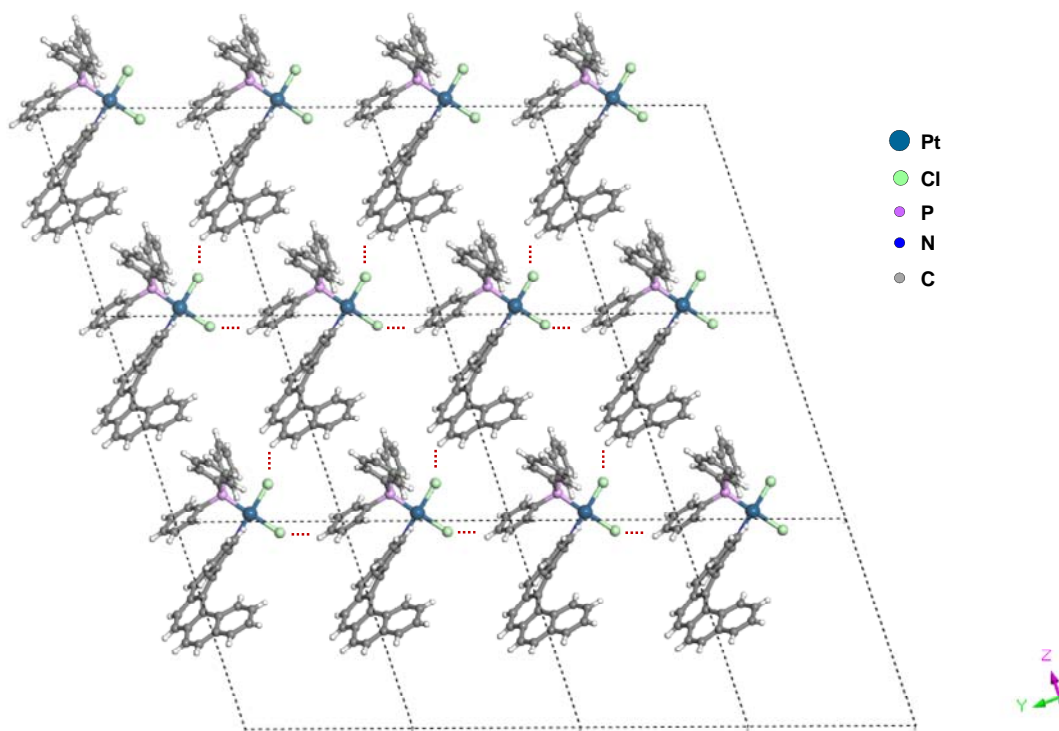
Figure 4. Arrangement of cis complex 4a in the yz plane. Hydrogen bonds between Cl and H atoms are emphasized in red.
