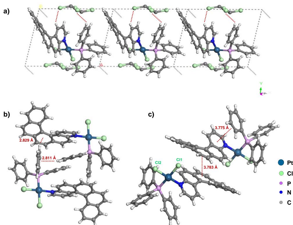
Figure 2. Crystal structure of 1 showing a) the arrangement along the x axis, with H-bonding interactions involving the CH 2 Cl 2 solvent molecules (disordered, two positions found), b) the intermolecular CH- \pi interactions and c) the inter/intramolecular \pi - \pi interactions between PPh 3 and the pyridyl cycle, and between the two central rings of two 4H5 in the heterochiral assembly of cis -PtCl 2 ( 4H5 )(PPh 3 ) ( 1 ) .
