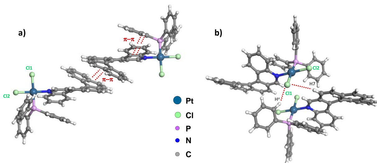
Figure 5. a) \pi - \pi interaction between helicenic rings of two adjacent heterochiral P - and M - 4a . b) Selected Cl \cdots H interactions between two heterochiral P - and M - 4a .
