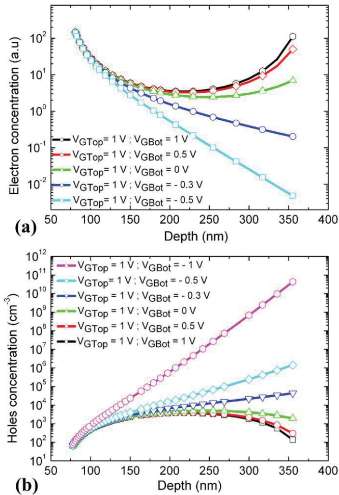
Fig. 9. Simulated distribution of electrons (a) at V_{Top}=1V ( V_{GBot}=-0.5 to 1V ) and holes (b) through a 300 nm width nanowire. Bottom channel conduction is as important as top channel's for positive bottom gate biasing.
