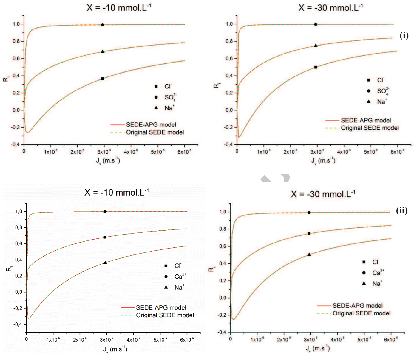
Figure 6. Comparison of the rejection rate against the volume flux using SEDE-APG and the original SEDE model. Figure (i) correspond to an electrolyte solution of 100 \text{ mol.L}^{-1} \text{ Na}_2\text{SO}_4 and 200 \text{ mol.L}^{-1} \text{ NaCl} . Figure (ii) correspond to an electrolyte solution of 100 \text{ mol.L}^{-1} \text{ CaCl}_2 and 200 \text{ mol.L}^{-1} \text{ NaCl} . In each figure, the results are represented for charge densities of -10 \text{ mmol.L}^{-1} and -30 \text{ mmol.L}^{-1} .
