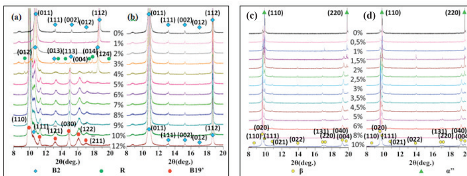
Fig. 2. SXRD patterns corresponding to the different incremental strain % under loading (a) and after each unloading (b) for NiTi. SXRD patterns corresponding to the different incremental strain % under loading (c) and after each unloading (d) for Ti-27Nb.
