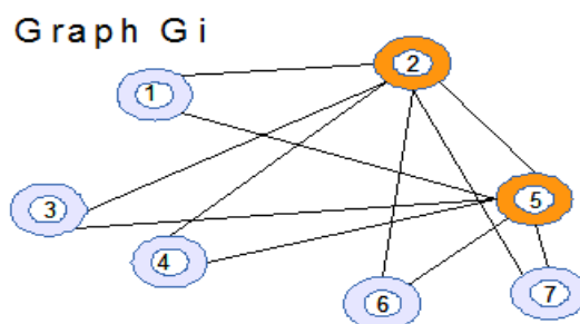
Figure 5. Nodes 2 and 5 are t_i -relevant as they have a maximum degree of n = 6 .
