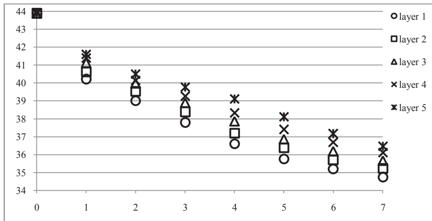
Fig.3. Time-courses of the porosity during 7 working days for each sand layer.
