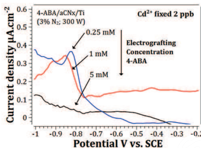
Figure 9: Electrochemical response in a DPASV mode for a benzoic acid modified a-CNx electrode using different diazonium salt concentrations (5 ; 1 and 0.25 mM ; 1 cycle). Acetate buffer 0.1 M and Cd 2+ 2 ppb; pH= 4.9 ; E step = 10 mV ; E pulse = 30 mV ; E dep = -1.1 V ; T dep =120 s ; V b = 50 mV s -1 .
