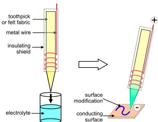
Figure 1. Scheme showing the principle of the EChemPen.
