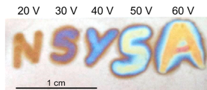
Figure 5. Titanium oxidation using the EChemPen.
