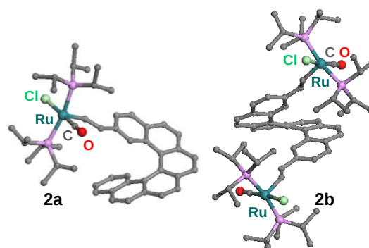
Figure 1. X-Ray crystallographic structure of 2a and 2b . Only P -enantiomers shown; H atoms omitted for clarity. [4a]
