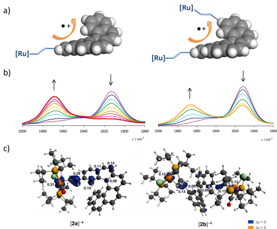
Figure 10. a) Schematic representation of helical radical cation grafted with one or two conjugated metal centers. b) IR region of the \nu(\text{CO}) stretch upon mono-oxidation of 2a and 2b . c) B3LYP/SV(P) electron spin density, \Delta\rho = \rho^\alpha - \rho^\beta (0.005 au), in [2a]⁺ and [2b]⁺ . Numbers listed are fractions of the total integrated spin density obtained from Mulliken decomposition of \Delta\rho . Compare SI.
