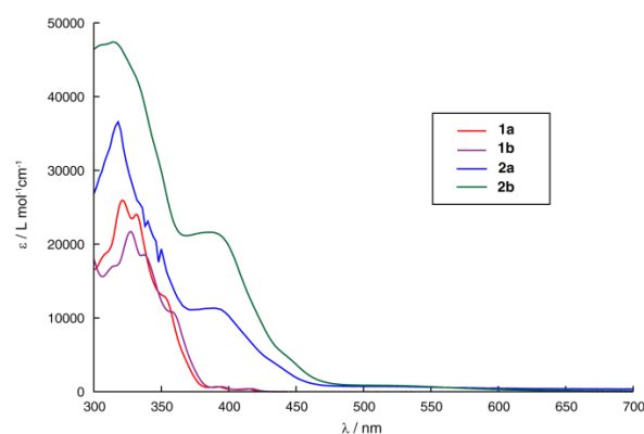
Figure 2. UV-vis spectra in CH 2 Cl 2 at 293 K of mono- and bis-ethynyl-helicenes 1a,b and of the corresponding mono- and bis-ruthenium-grafted vinylhelicene derivatives 2a,b .
