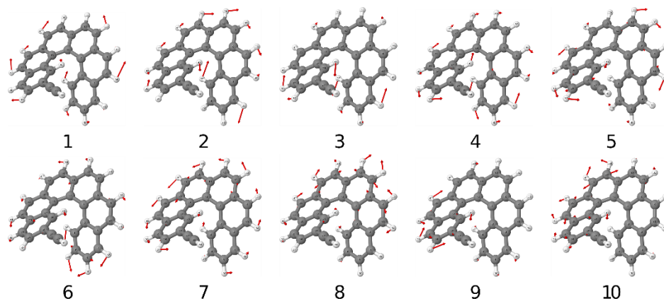
Figure 8. Atomic displacements for selected normal modes in 1a .
