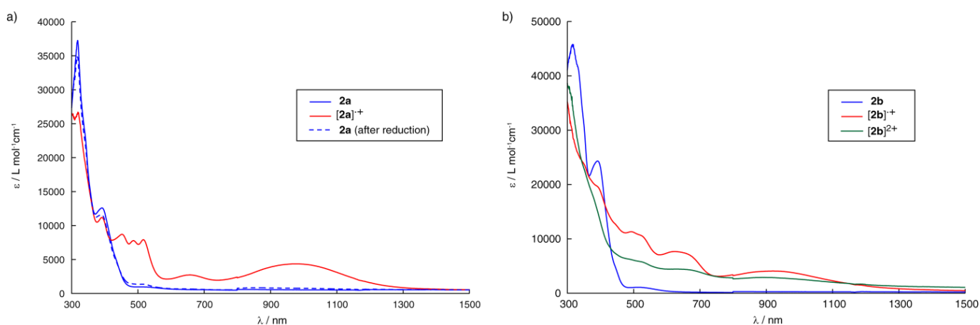
Figure 11. UV-vis/NIR spectroelectrochemistry: a) oxidation at 0.4 V (vs. Fc/Fc⁺) of complex 2a in DCE / 0.2 M [NBu₄]⁺[PF₆]⁻ at r.t., followed by reduction at -0.4 V (vs. Fc/Fc⁺), and b) first and second oxidation of complex 2b in DCE / [NBu₄]⁺[PF₆]⁻ at r.t..
