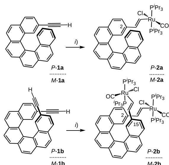
Scheme 1. Synthesis of enantiopure P - and M - ruthenium-grafted vinylhelicene derivatives 2a,b . i) RuH(CO)Cl(P i Pr 3 ) 2 , CH 2 Cl 2 or toluene, r.t., Ar.
