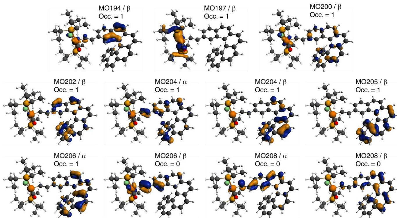
Figure 13. Isosurfaces (0.05 au) of MOs involved in selected transitions of [2a]^+ .
