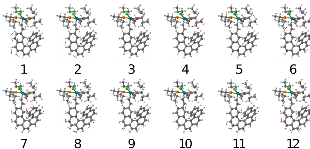
Figure 8. Atomic displacements for selected normal modes in 1a .
