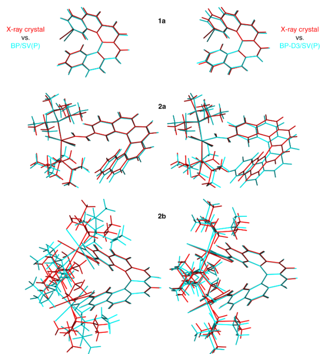
Figure 5. Overlays of calculated BP/SV(P), BP-D3/SV(P), and experimental X-ray crystal structures of 1a , 2a , and 2b .
