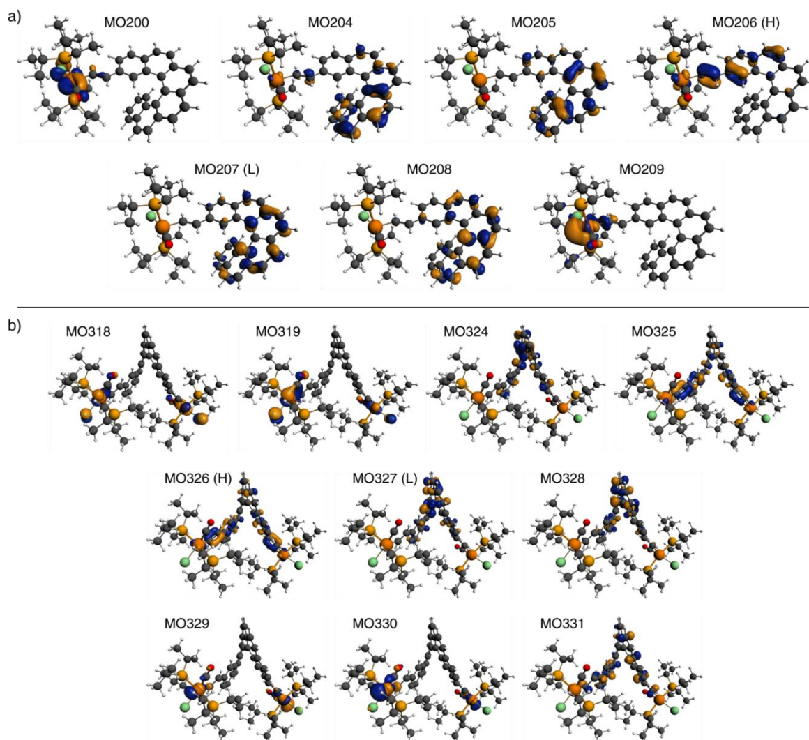
Figure 4. Isosurfaces (0.05 au) of MOs involved in selected transitions of 2a (panel a) and 2b (panel b). 'H' = HOMO, 'L' = LUMO.
