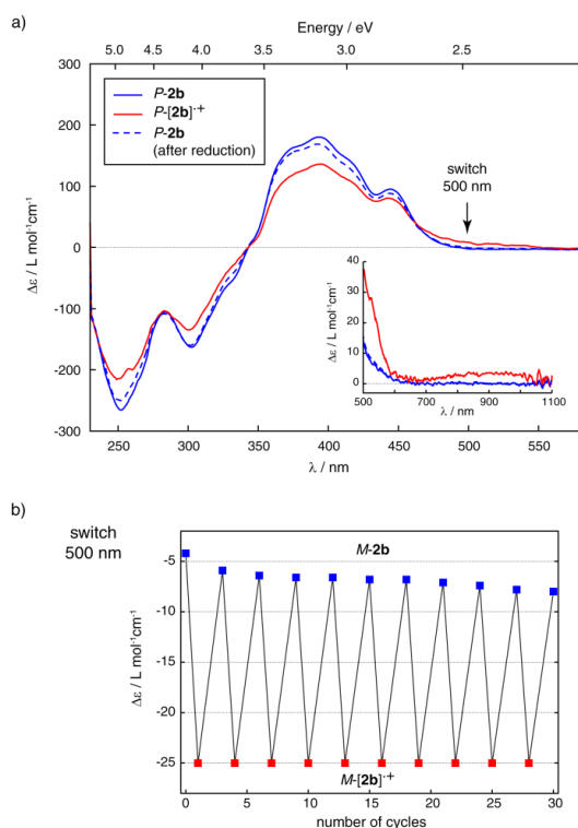
Figure 14. a) Experimental CD spectra of enantiopure P -(+)- 2b and of its oxidized (DCE, r.t.) species P -(+)- [2b]^+ . Dashed line indicates CD spectra for P -(+)- 2b obtained via reduction of P -(+)- [2b]^+ . Inset: NIR CD spectra of P -(+)- 2b and P -(+)- [2b]^+ . b) Redox chiroptical switching M -(−)- 2b \leftrightarrow M -(−)- [2b]^+ observed by CD spectroscopy at 500 nm. Compare Figure S10, SI.
