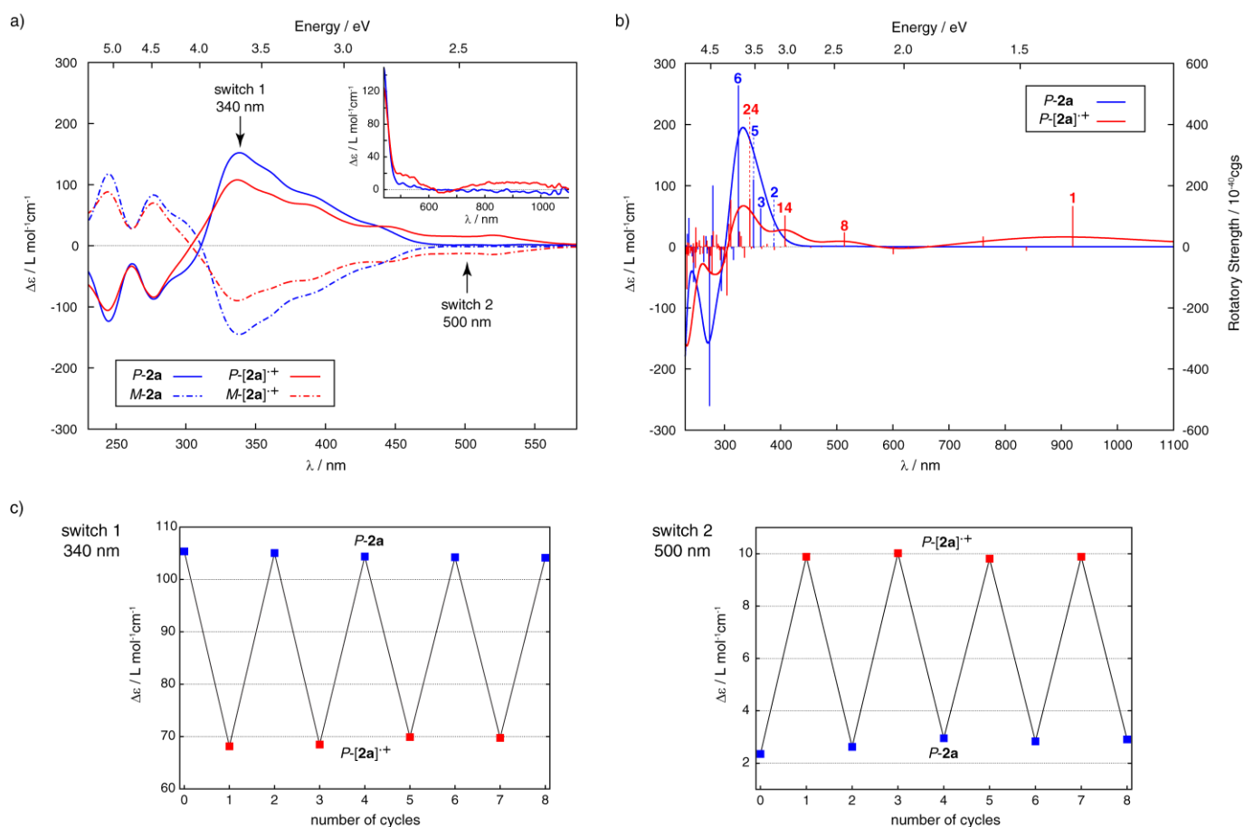
Figure 12. a) Experimental CD spectra of P -(+)- and M -(-) enantiomers of 2a and of their oxidized (DCE, r.t.) species [2a] + . Inset: NIR CD spectra of P -(+)- 2a and P -(+)-[2a] + . b) Calculated B3LYP/6-31G(d,p) TDDFT ECD spectra of P -(+)- 2a and P -(+)-[2a] + . No spectral shift has been applied. Numbered excitations correspond to those analyzed in detail in Table 1 and Table 6. c) Dual redox chiroptical switching P -(+)- 2a ↔ P -(+)-[2a] + observed by ECD spectroscopy at 340 and 500 nm.
