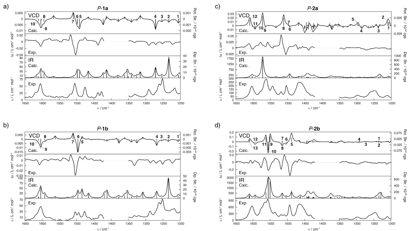
Figure 7. Comparison of experimental (dichloromethane) vs. calculated B3LYP-D3/SV(P) (gas-phase, frequencies scaled by 0.9614) IR and VCD spectra for P - 1a (panel a), P - 1b (b), P - 2a (c), and P - 2b (d). Numbered VCD vibrations correspond to those analyzed in detail.
