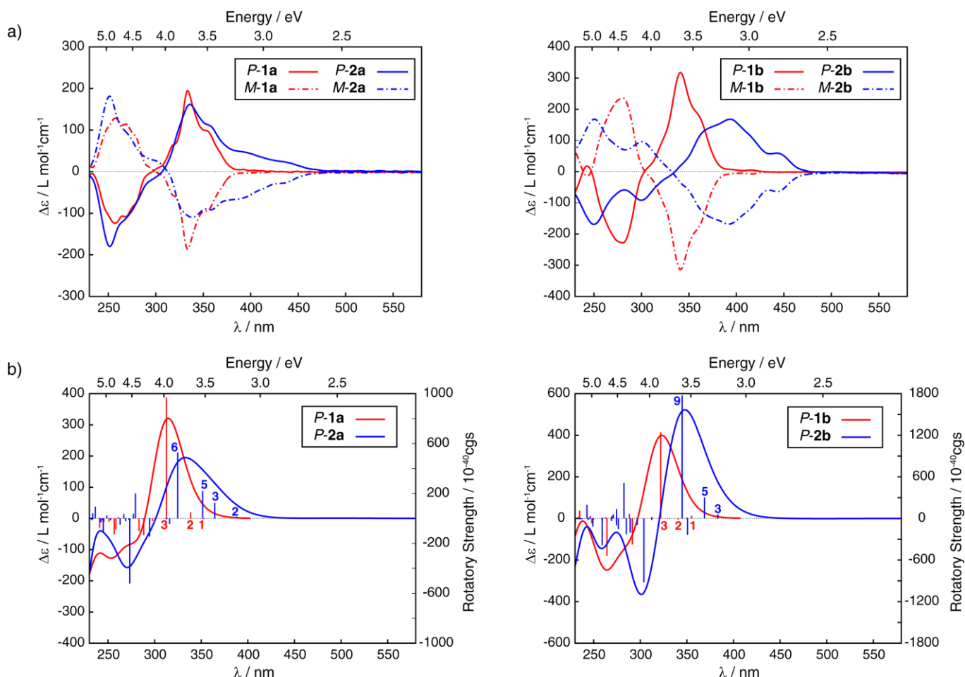
Figure 3. ECD spectra in \text{CH}_2\text{Cl}_2 at 293 K of a) enantiopure mono-alkynyl precursors P -(+)- and M -(-)- 1a and the corresponding mono-ruthenium-grafted vinyl-helicene derivatives P -(+)- and M -(-)- 2a and of b) enantiopure bis-alkynyl precursors P -(+)- and M -(-)- 1b and the corresponding bis-ruthenium-grafted vinyl-helicene derivatives P -(+)- and M -(-)- 2b (top panels). In the bottom panels the corresponding simulated B3LYP/SV(P) TDDFT ECD spectra are shown. No spectral shift has been applied. Numbered excitations correspond to those analyzed in detail in Table 1 and SI.
