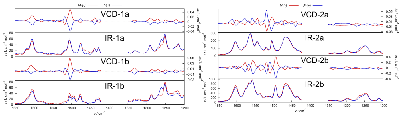
Figure 6. Experimental IR and VCD spectra for P -(+) and M -(-) mono- and bis-alkynylhelicenes ( 1a , b ) and P -(+) and M -(-) mono- and bis-ruthenium-vinylhelicenes ( 2a , b ). VCD spectra measured in \text{CD}_2\text{Cl}_2 at 293 K (concentrations \sim 15 mg in 0.7 mL; 0.5 mm pathlength; 3000 scans).
