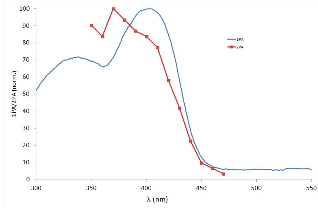
1PA (blue) and 2PA (red) spectra (plotted against half of the excitation wavelength) of 5 in dichloromethane.
