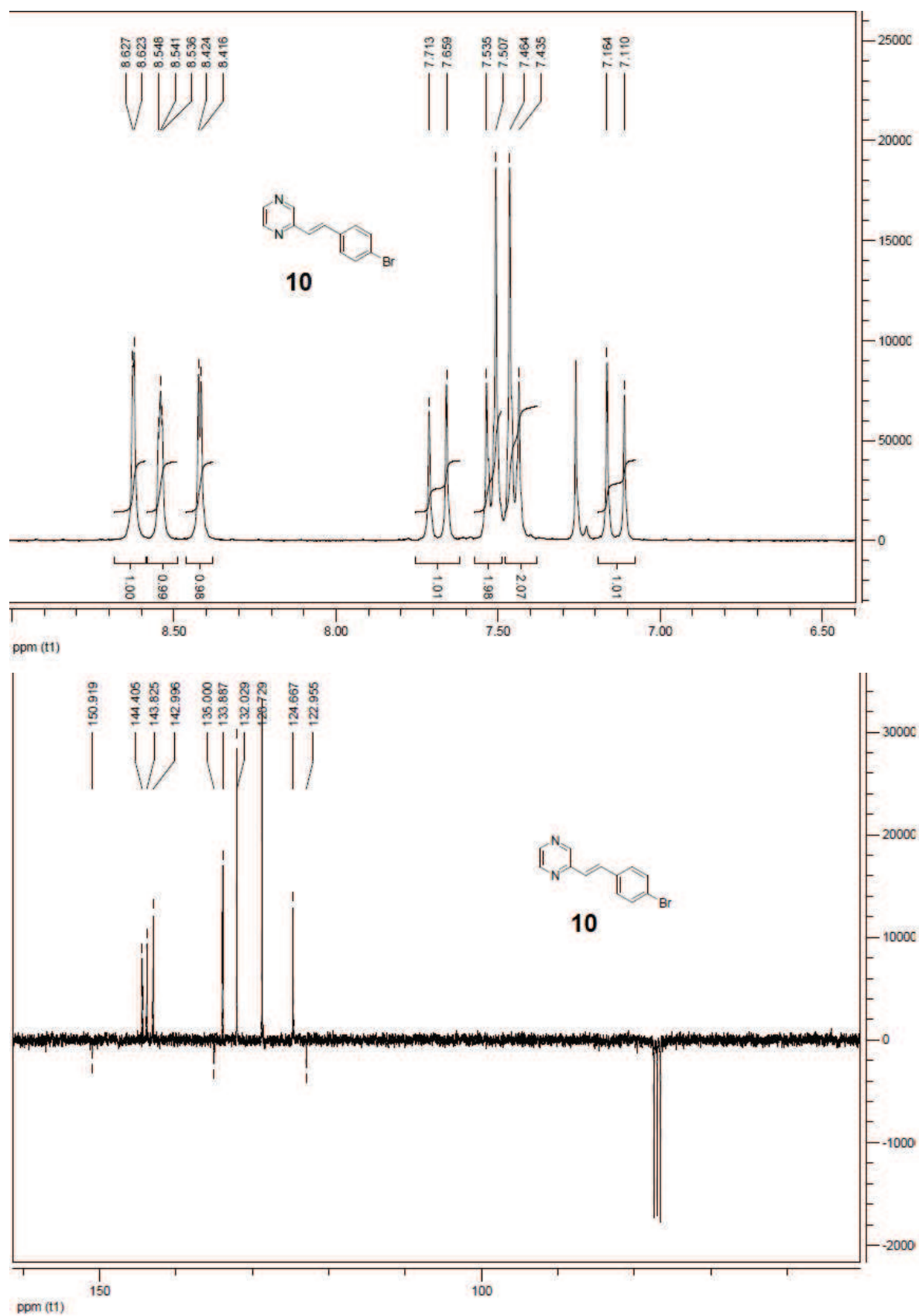
1 H and 13 C-NMR spectra of intermediate 10 (300/75 MHz, CDCl 3 ).
