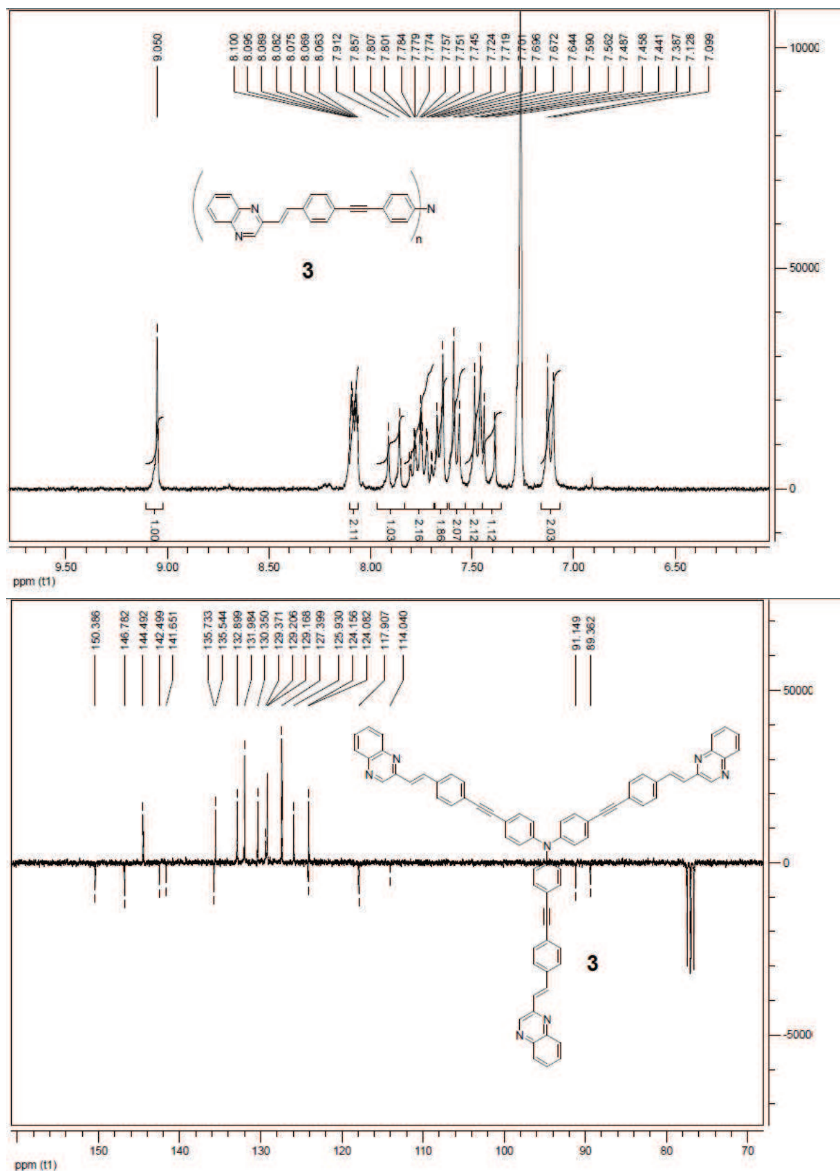
^1\text{H} and ^{13}\text{C} -NMR spectra of chromophore 3 (300/75 MHz, \text{CDCl}_3 ).
