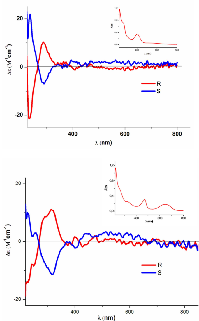
Fig. 7. CD spectra in CH 2 Cl 2 (inserts: UV-vis absorption spectra) of neutral complex 2 (top) and monooxidized complex [2][TCNQ] . (bottom).
