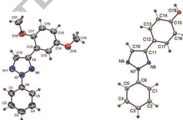
Figure 2. ORTEP diagram (50% probability) of 4d and 4e .
