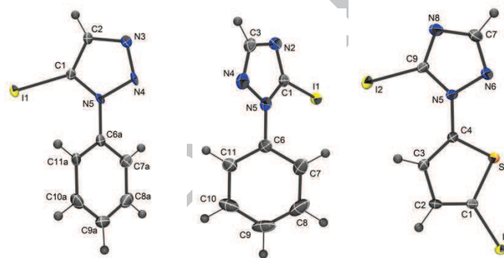
Figure 1. ORTEP diagram (50% probability) of 5a , 6a and 7b .
