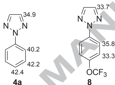
Scheme 10. Comparison of \text{pK}_a(\text{THF}) values of 4a vs 8 .
