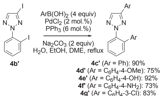
Scheme 8. Suzuki-type cross-coupling from 4b' .
