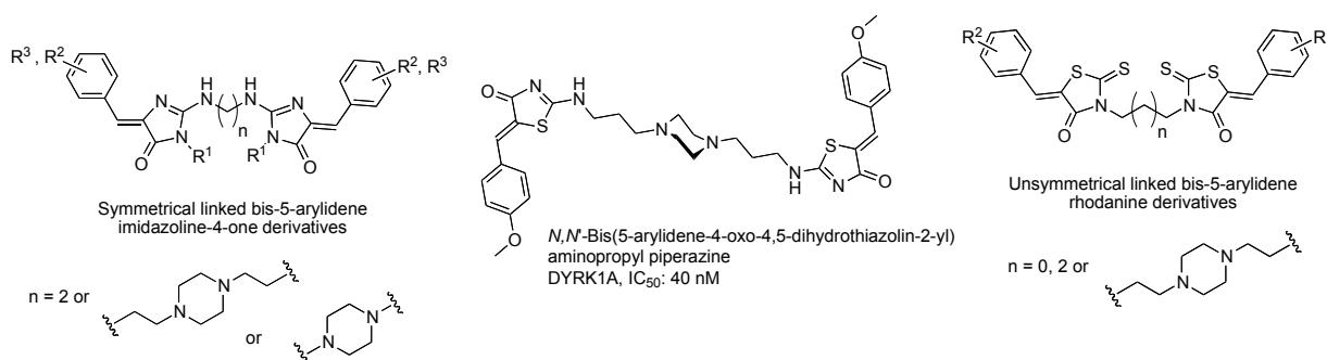
Figure 1. Symmetrical linked bis-5-arylidene imidazoline-4-ones, symmetrical linked bis-5-arylidene-1,3-thiazoline-4-ones and unsymmetrical linked bis-5-arylidene rhodanines derivatives (as inhibitors of the protein kinase DYRK1A or against cell proliferation on cell tumor lines) identified and developed in our group.
