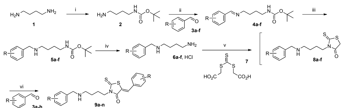
Scheme 1. Route used for the preparation of 3-(4-arylmethylamino)butyl-5-arylidene-2-thioxo-1,3-thiazolidine-4-ones 9 via the “one-pot two-steps” reaction under microwave. Reagents and reaction conditions: (i) (t\text{-BuO}_2\text{C})_2\text{O} , 1,4-dioxane, 25\text{ }^\circ\text{C} , 24 h. (ii) 3 1 equiv., molecular sieve 3\text{\AA} , \text{Et}_2\text{O} , 25\text{ }^\circ\text{C} , 16 h. (iii) \text{NaBH}_4 5 equiv., MeOH, 50\text{ }^\circ\text{C} , 24 h. (iv) HCl 6 M, 1,4-dioxane, 25\text{ }^\circ\text{C} , 4 h. (v) 6 1 equiv., 7 1 equiv., \text{Et}_3\text{N} 2 or 3 equiv., DME, MWI, 90\text{ }^\circ\text{C} , 15 or 30 min. (vi) 3 1 equiv., MWI, 110\text{ }^\circ\text{C} , 15 or 30 min.
