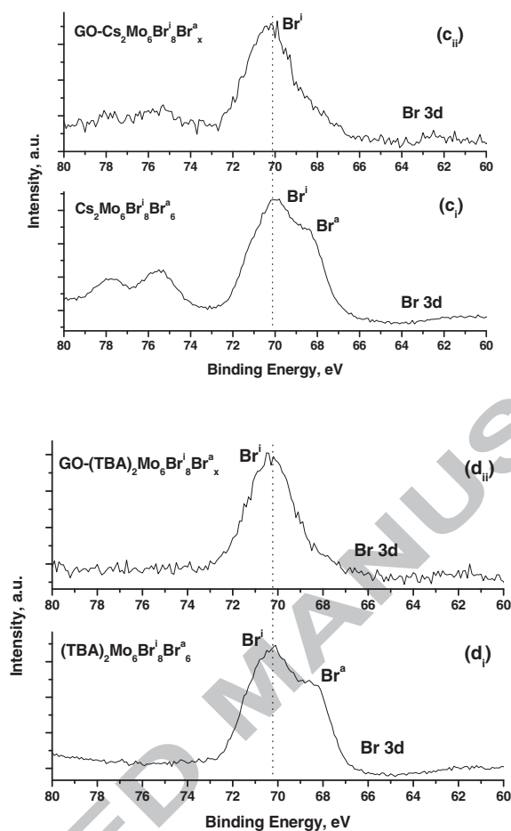
Fig 4: XPS spectra of (a) Cs 3d; (b) Mo 3d; (c) Br 3d regions for \text{Cs}_2\text{Mo}_6\text{Br}_8\text{Br}_x^a and \text{GO-Cs}_2\text{Mo}_6\text{Br}_8\text{Br}_x^a ; (d) Br 3d regions for (\text{TBA})_2\text{Mo}_6\text{Br}_8\text{Br}_x^a and \text{GO-(TBA)}_2\text{Mo}_6\text{Br}_8\text{Br}_x^a composites.
