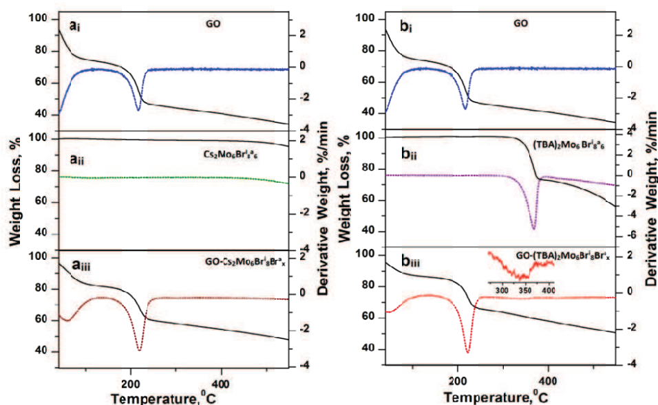
Fig 5: TG-DTA patterns of (a) GO, \text{Cs}_2\text{Mo}_6\text{Br}_8^i\text{Br}_6^a cluster and \text{GO-Cs}_2\text{Mo}_6\text{Br}_8^i\text{Br}_x^a composite; (b) GO, (\text{TBA})_2\text{Mo}_6\text{Br}_8^i\text{Br}_6^a cluster and \text{GO-(TBA)}_2\text{Mo}_6\text{Br}_8^i\text{Br}_x^a composite over the temperature range of 30-550 °C under nitrogen flow.
