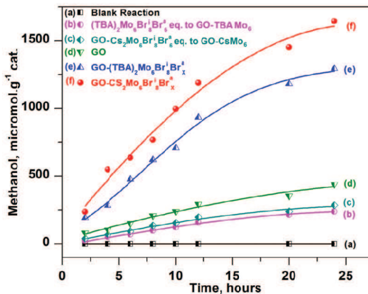
Fig 7: Methanol formation rate in (a) blank reaction, (b, c) using (TBA) 2 Mo 6 Br 8 Br 6 a and Cs 2 Mo 6 Br 8 Br 6 a in equimolar amounts as presented in GO-composites, (d) GO, (e) GO-(TBA) 2 Mo 6 Br 8 Br 6 a and (f) GO-Cs 2 Mo 6 Br 8 Br 6 a catalyzed photoreduction of CO 2 .
