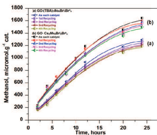
Fig: 8 Recycling experiments using (a) GO- (TBA) 2 Mo 6 Br 8 i Br x a and (b) GO- Cs 2 Mo 6 Br 8 i Br x a .
