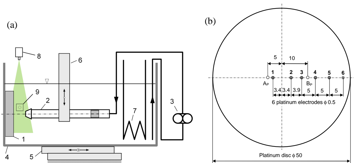
Fig. 1 a): Diagram of apparatus: 1 target disc with electrodes, 2 tube with nozzle and honeycomb, 3 pump, 4 reservoir, 5 compound table, 6 nozzle holder, 7 cooling coil, 8 laser source with laser sheet in the mild plane of the nozzle, 9 FlowSense EO camera b): Target disc with electrodes row: 1-6 electrodes \phi 0.5mm. A_P and B_P are the limits of stagnation point displacement.
