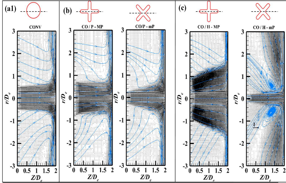
Fig.5 Mean vector fields \left(\frac{W}{W_0} \vec{e}_z + \frac{U_r}{W_0} \vec{e}_r\right) and the corresponding streamlines (in blue): convergent nozzle (a), cross-shaped orifice on a plane (b), cross-shaped orifice on a hemisphere (c)
