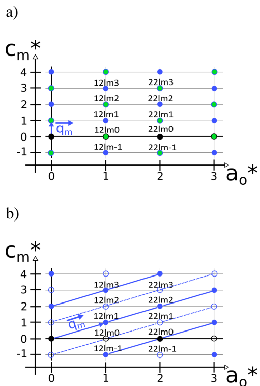
Figure 5 a) Schematic representation of the (\mathbf{a}^*, \mathbf{c}^*) diffraction plane for h=2 in the phase III of n -tetracosane/urea: black points refer to structure Bragg peaks of the high symmetry phase, green and blue points indicate the positions of Bragg peaks which sign the supplementary modulation; b) schematic representation of the same diffraction plane in the phase II: black points refer to structure Bragg peaks of the high symmetry phase, blue points indicate the positions of Bragg peaks which appear in this phase II.
