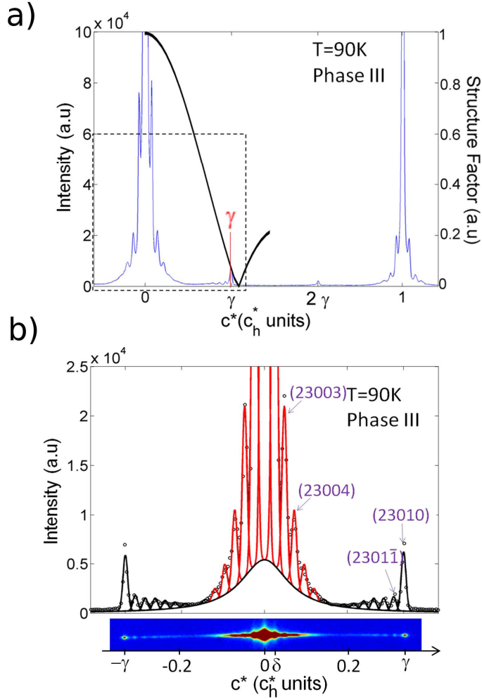
FIG. 4. a) n -Tetracosane/urea (2\ 3\ 0\ m\ n)_o superstructure line (in blue) measured at 90 K on the CRISTAL beamline at SOLEIL along the incommensurate direction in the q range of -0.2c_h^* to 1.2c_h^* in reciprocal urea units; Inset in black: Molecular form factor of the n -tetracosane molecule aligned along the c direction with six-fold orientational disorder, as calculated in [39]. b) Diffraction image and extracted profile of the (2\ 3\ 0\ m\ n)_o superstructure line between -0.4c_h^* and +0.4c_h^* . Superstructure satellite Bragg peaks are associated with a critical wave vector q_i = \pm (0.025 \pm 0.001)c_h^* . Satellite peaks were fit using Gaussians and are indexed as (2\ 3\ 0\ 0\ m)_o in red and (2\ 3\ 0\ 1\ m)_o in
