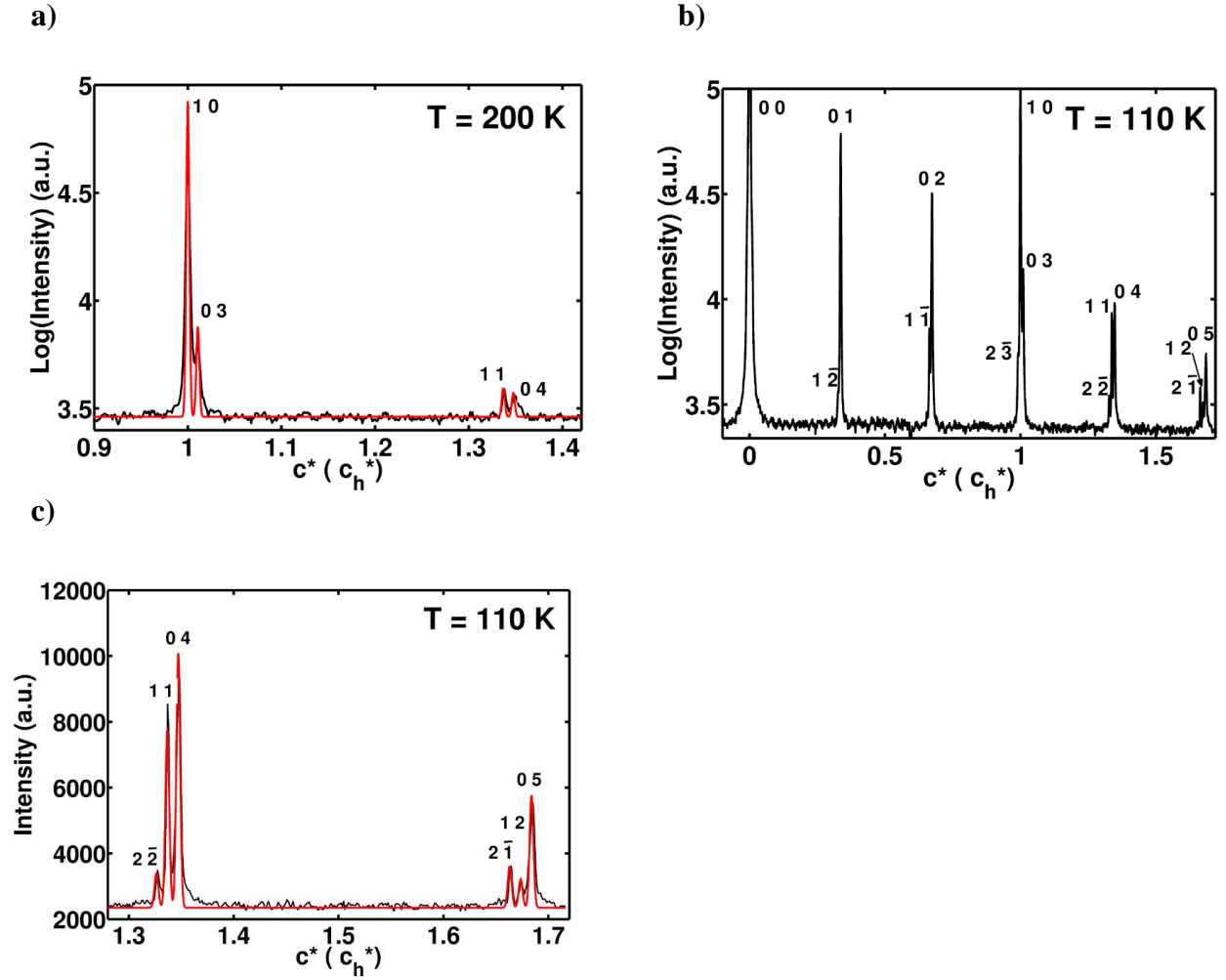
FIG. 2. Profiles along c^* using a detector distance of 980 mm on beamline 14-BM-C at the APS. a) Profile (logarithmic intensity scale) and fit of a section of the the (1\ 0\ l\ m)_h layer line of Phase I at 200 K with \gamma = 0.3369 \pm 0.0005 . The l and m indices are shown next to each peak. b) Profile (logarithmic intensity scale) of the equivalent (0\ 2\ l\ m\ n)_o layer line of Phase III at 110 K showing the values of l and m for each assigned peak. (In this structure line, n = 0 in all cases.) c) An enlargement of the profile of the (0\ 2\ l\ m\ n)_o layer line of Phase III at 110 K from Q(c_h^*) of 1.3 to 1.7 (linear intensity scale) showing the l and m indices and the corresponding fit with \gamma = 0.3369 \pm 0.0002 . In these structure lines at 200 and 110 K, all of the Bragg peaks can be fit with Gaussian functions at the combinatory positions for l and m .
