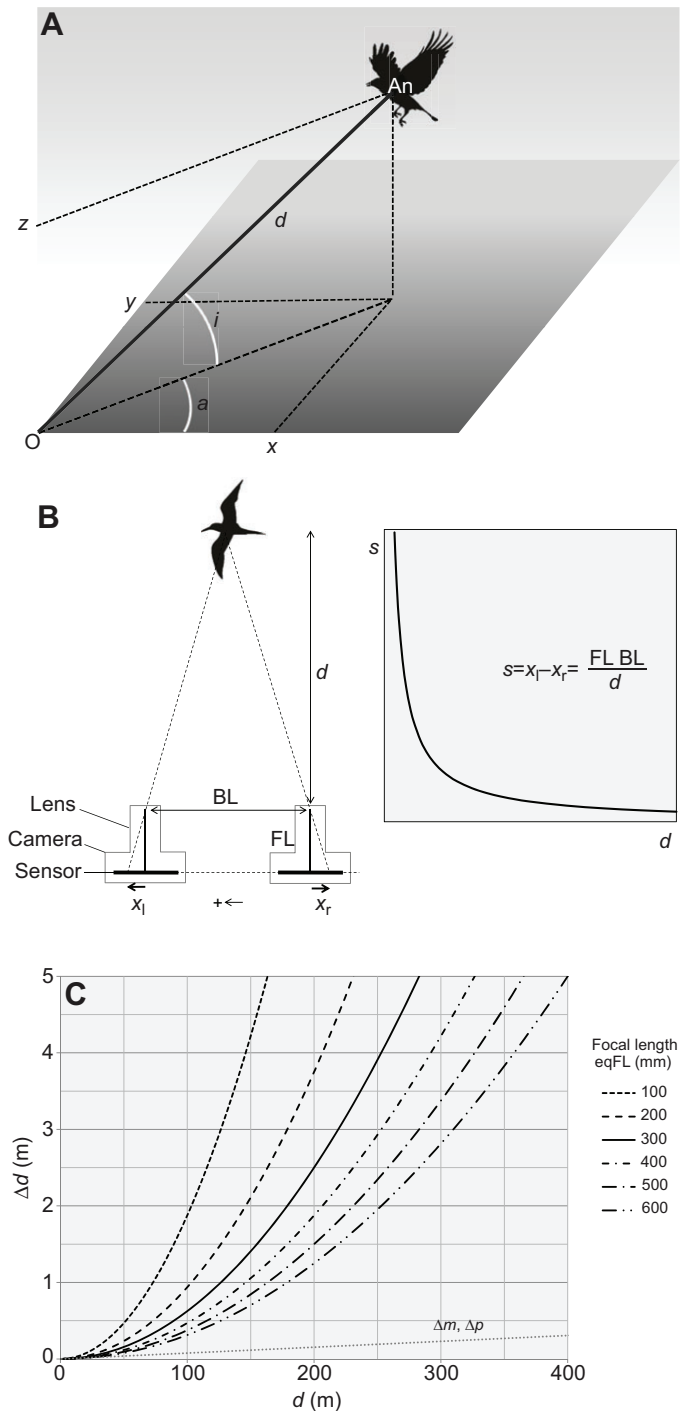
Fig. 1. Geometric principles of the tracking method. (A) The position of the animal (An) relative to the observer (O) is measured using spherical coordinates, i.e. azimuth angle ( a ), inclination angle ( i ) and distance ( d ). (B) The basic principle of distance ( d ) measurement from stereo images. BL, base length separating dual cameras; FL, focal length; x l , x r , position of the animal image on the left and right images, respectively. The lateral shift ( s ) between stereo images is an inverse function of distance. (C) Plots of the distance resolution ( \Delta d ), as a function of distance ( d ), for BL=1 m, IW=1920 pixels and various focal lengths (eqFL). \Delta d grows quadratically with increasing distance, limiting the range of precise tracking. The linear resolutions due to the angular digital measurement ( \Delta m and \Delta p , for 13 bit digital rotary encoders) are also plotted for comparison.
