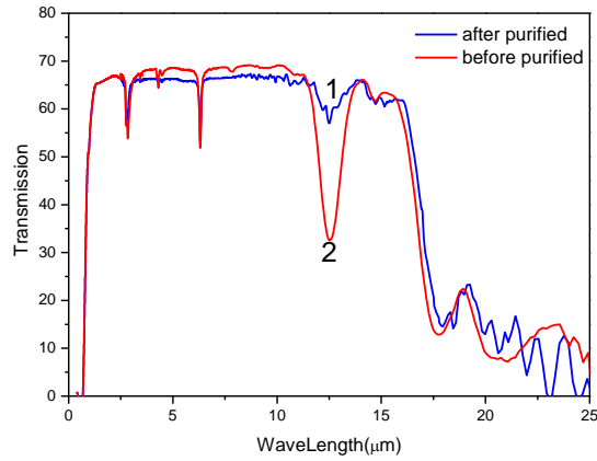
Fig. 7. Optical transmission spectra of \text{Ge}_{20}\text{Sb}_5\text{Se}_{55}\text{I}_{20} glasses (2 mm thick) (1) glass purified with Mg getter and (2) glass without purification
