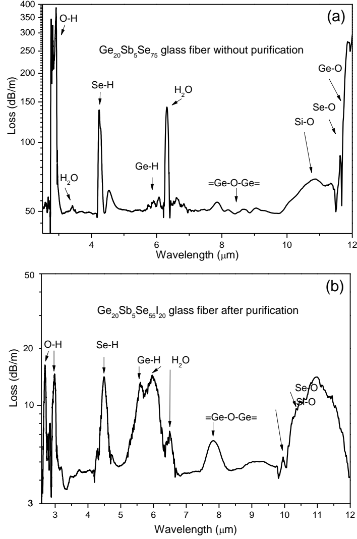
Fig. 8. Transmitting loss spectra of (a) \text{Ge}_{20}\text{Sb}_5\text{Se}_{75} and (b) \text{Ge}_{20}\text{Sb}_5\text{Se}_{55}\text{I}_{20} fibers
