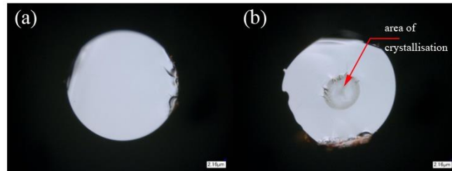
Fig. 8. Drawn fiber end under the digital microscope:
