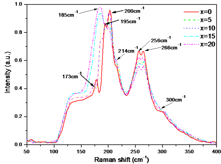
Fig. 5. Normalized Raman spectra of the \text{Ge}_{20}\text{Sb}_5\text{Se}_{75-x}\text{I}_x glasses
