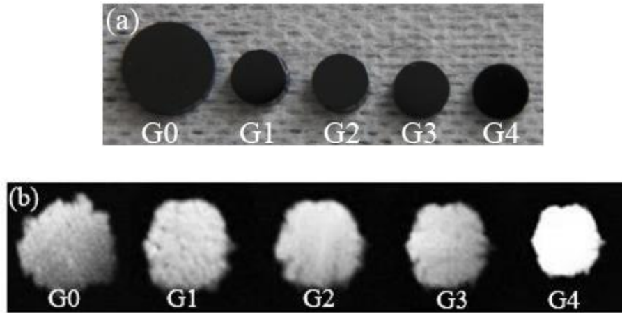
Fig. 1. (a) Visible region images and (b) images of stripes in different glasses taken with an NIR imaging camera operating at a wavelength of 1\ \mu\text{m}
