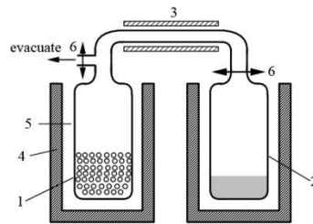
Fig. 6. The setup for glass preparation:
