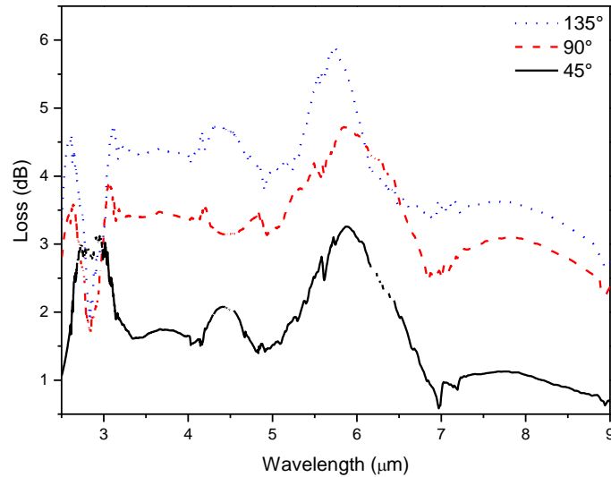
Fig. 9. Bend loss spectra of the \text{Ge}_{20}\text{Sb}_5\text{Se}_{55}\text{I}_{20} optical fiber
