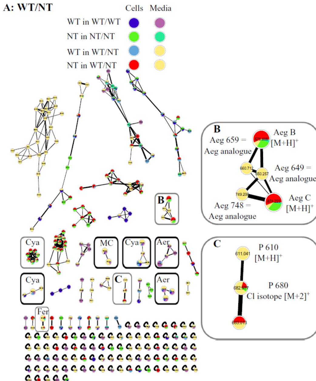
Fig. 5. A) WT and NT intra- and extracellular molecular network under mono- (WT/WT, NT/NT) and WT/NT co-culture conditions. Larger circles indicate matches with the GNPS library. B) Molecular network of MS/MS spectra of aeruginosamide variants. Compounds produced by WT are in black rectangles and those produced by NT are in grey ones. C) Molecular network of MS/MS spectra of unknown peptides.
