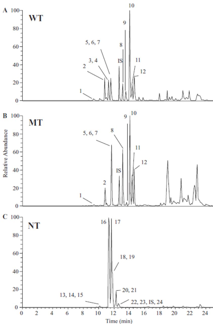
Fig. 1. Chromatograms obtained for WT (A), MT (B) and NT (C) in monoculture. Peaks legend (full names are given in Table 2): 1- Arg 684, 2- Aer D, 3- Des-MCLR, 4- MCLR, 5- Cya B, 6- Cya C, 7- Cya A, 8- Cya 963A, 9- Cya 895, 10- Aer A, 11- Aer C, 12- Aer B, 13- P 612, 14- P 646, 15- P 680, 16- Aeg B, 17- Aeg C, 18- Fer A, 19- Fer B, 20- Cya 964, 21- Cya 978, 22- Cya 914, 23- Cya 948, 24- Cya 962, IS: Internal Standard (retention time = 12.6 min).
