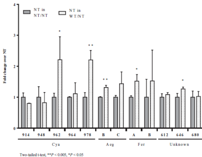
Fig. 2. Relative concentrations given as a fold change over WT ( A ) or NT ( B ) in monoculture of selected intracellular compounds for WT, MT and NT strains under mono- (WT/WT, MT/MT, NT/NT) and co-culture (WT/MT, WT/NT) conditions and statistical results. MC: Microcystin, Arg: Aeruginosin, Cya: Cyanopeptolin, Aer: Aerucyclamide, Aeg: Aeruginosamide, Fer: Ferintoic acid.
