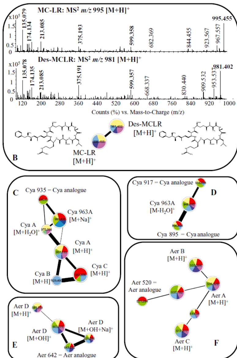
Fig. 4. A) WT and MT intra- and extracellular molecular network under mono- (WT/WT, MT/MT) and WT/MT co-culture conditions. Larger circles indicate matches with the GNPS library. B) Molecular network of MS/MS spectra of microcystin variants: MC-LR ( m/z 995) and Des-MCLR ( m/z 981). C) and D) Molecular network of MS/MS spectra of cyanopeptolin variants with the common structure Ahp-Leu-MePhe. E) and F) Molecular network of MS/MS spectra of aerucyclamide variants.
