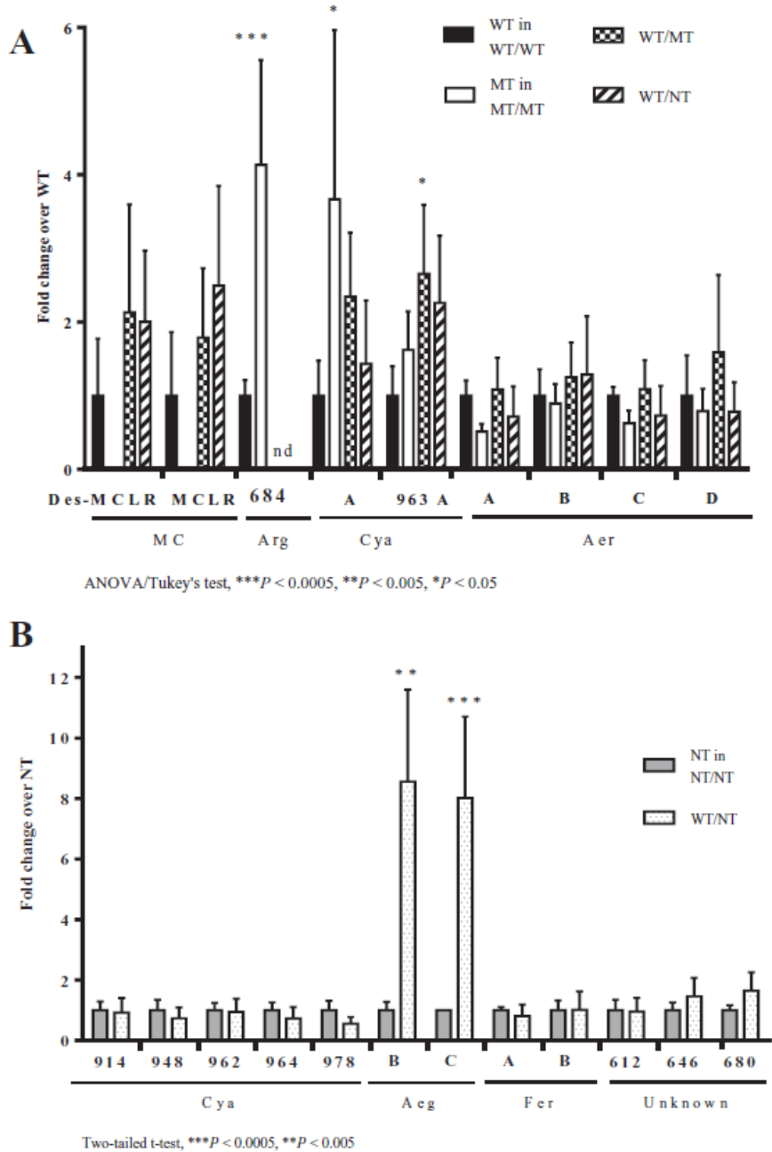
Fig. 3. Relative concentrations given as a fold change over WT ( A ) or NT ( B ) in monoculture of selected extracellular compounds for WT, MT and NT strains under mono- (WT/WT, MT/MT, NT/NT) and co-culture (WT/MT, WT/NT) conditions and statistical results. MC: Microcystin, Arg: Aeruginosin, Cya: Cyanopeptolin, Aer: Aerucyclamide, Aeg: Aeruginosamide, Fer: Ferintoic acid, nd: not detected.
