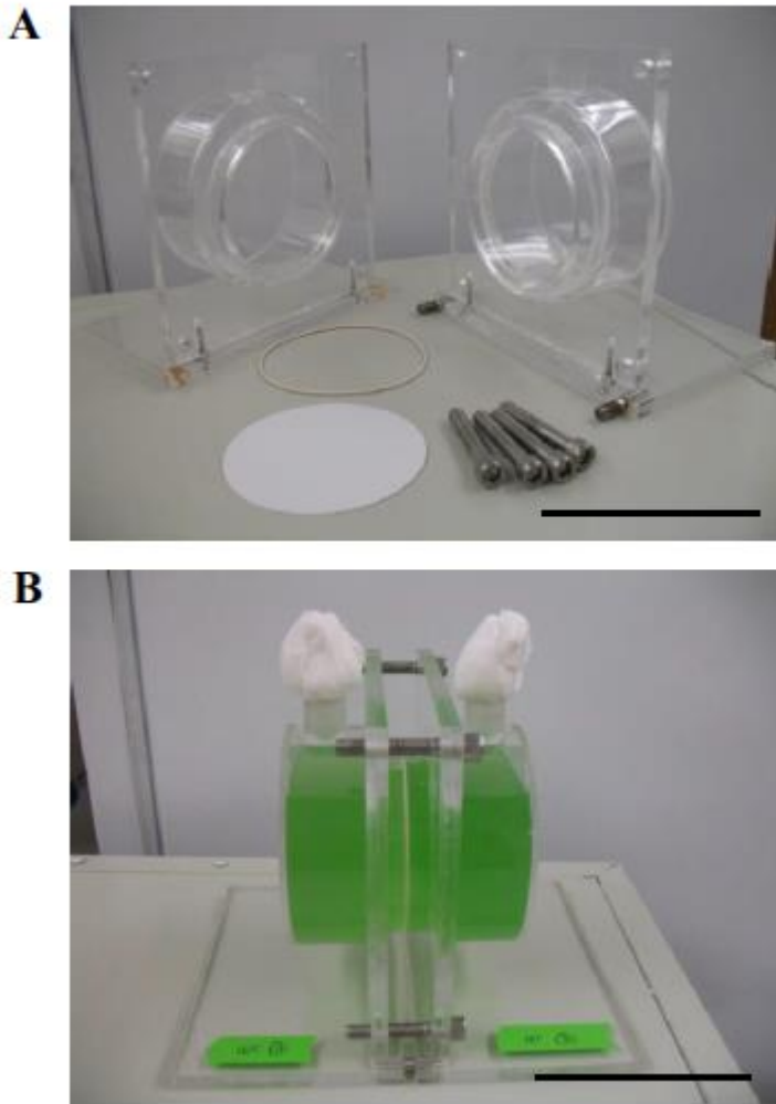
Fig. 6. Co-culture device to grow strains without physical contact but ensuring the exchange of dissolved solutes including secondary metabolites. A) The disassembled device with all parts required for the setup, and B) the assembled co-culture device. A 0.45\ \mu\text{m} membrane separates both chambers that can each be filled with up to 425 ml medium. The two chambers were held together by four screws and sealed with an O-ring. Each culturing chamber had a 20 mm opening at the top for filling and sampling purposes. The black bar represents 10 cm.
