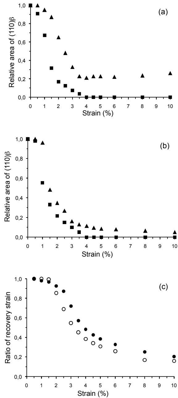
Fig. 9. Evolution of the relative area of the (110)_\beta peak during loading (square) and unloading (triangle) as a function of the applied strain for Ti-24Nb-0.5N alloy (a) and for Ti-24Nb-0.5O alloy (b); evolution of the ratio of recovery strain (c) for both Ti-24Nb-0.5N (black circles) and Ti-24Nb-0.5O (open circles) alloys.
