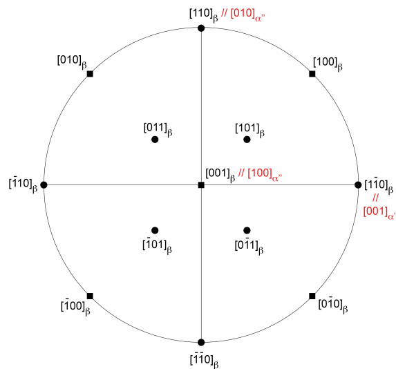
Fig. 8. Stereographic projection of the predominant orientation of \beta grains in the specimen; the tensile direction is along the [110]_{\beta} direction and the X-ray incident beam is along the [001]_{\beta} direction.
