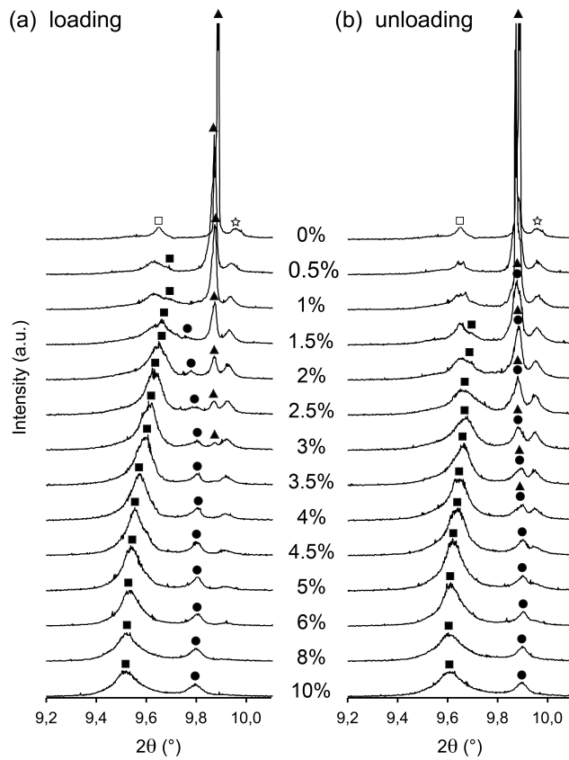
Fig. 5. SXR D patterns zoomed around the \{110\}_{\beta} peak (black triangles) acquired during the in situ cyclic tensile test under loading (a) and after unloading (b) for the Ti-24Nb-0.5N alloy; for each cycle, the corresponding strain is indicated beside each pattern. Squared symbols label the (020)_{\alpha''} peaks, circles label the (002)_{\alpha''} peaks and stars label the (111)_{\alpha''} peaks; open symbols correspond to the \alpha'' phase formed on quenching.
