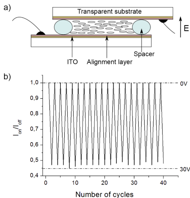
Figure 5. a) Representation of a planar-aligned LC cell. The molecular orientation within the cell corresponds to the OFF state; b) Evolution of the integrated photoluminescence signal of \text{Kat}_2[\text{Mo}_6\text{I}_{14}]:\text{E44} (1/9) mixture filled up in a planarly aligned LC cell upon irradiation at 400 nm and application (ON state) or not (OFF state) of a 30 V AC voltage at 78°C.
