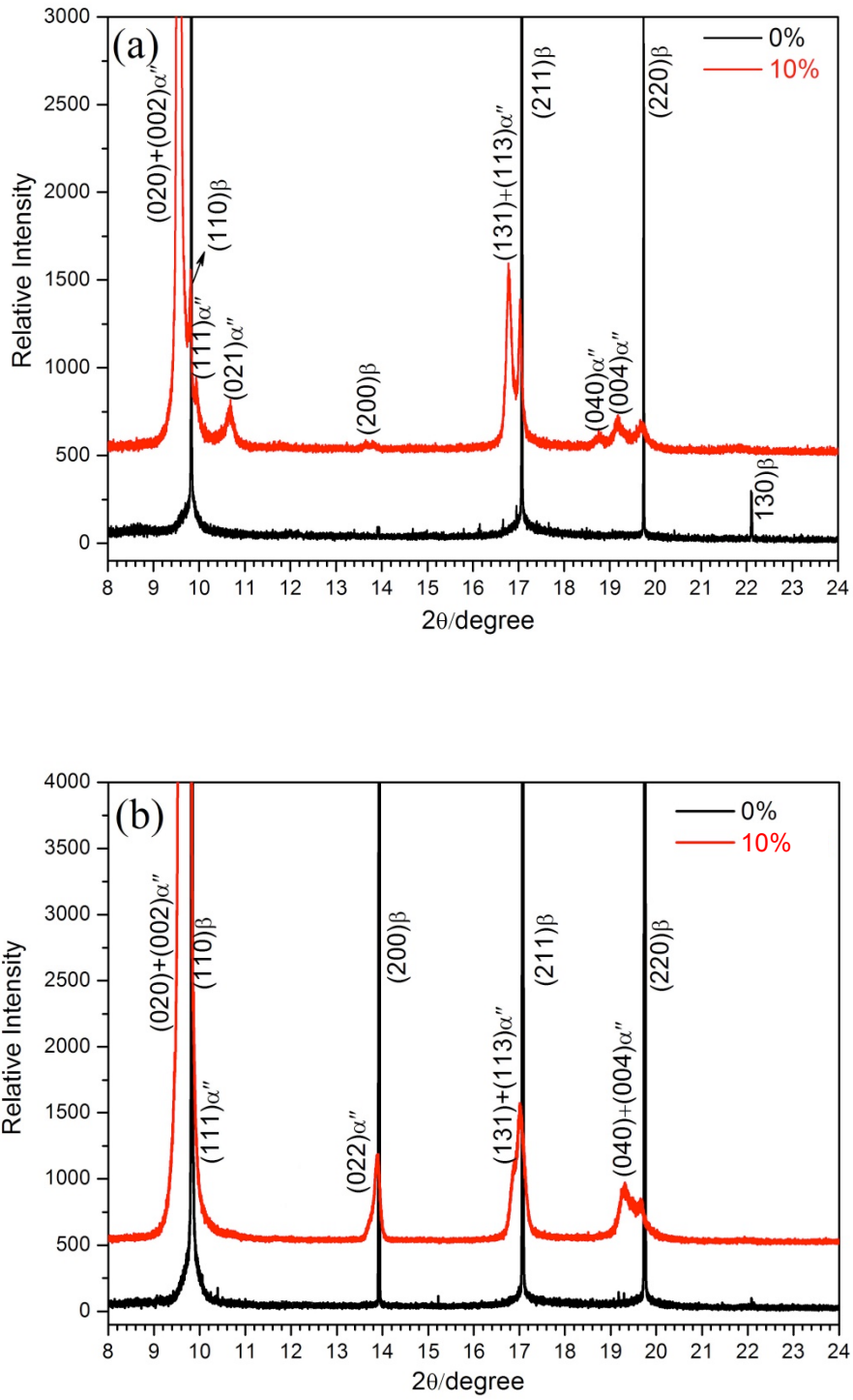
Fig. 3. In situ SXR D spectra of the Ti2448 alloy before deformation and after to be deformed at 10% of strain for ST (a) and FT (b).
