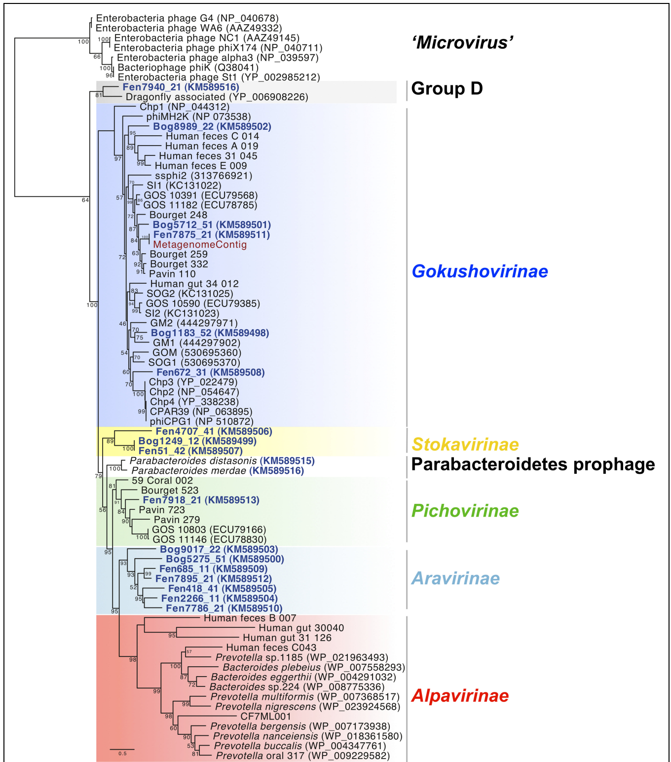
FIGURE 1 | Maximum likelihood phylogenetic analysis of full-length major capsid protein sequences present in the Microviridae genomes from Sphagnum-dominated peat viromes. A total of 253 unambiguously aligned positions from 76 sequences were used in the
