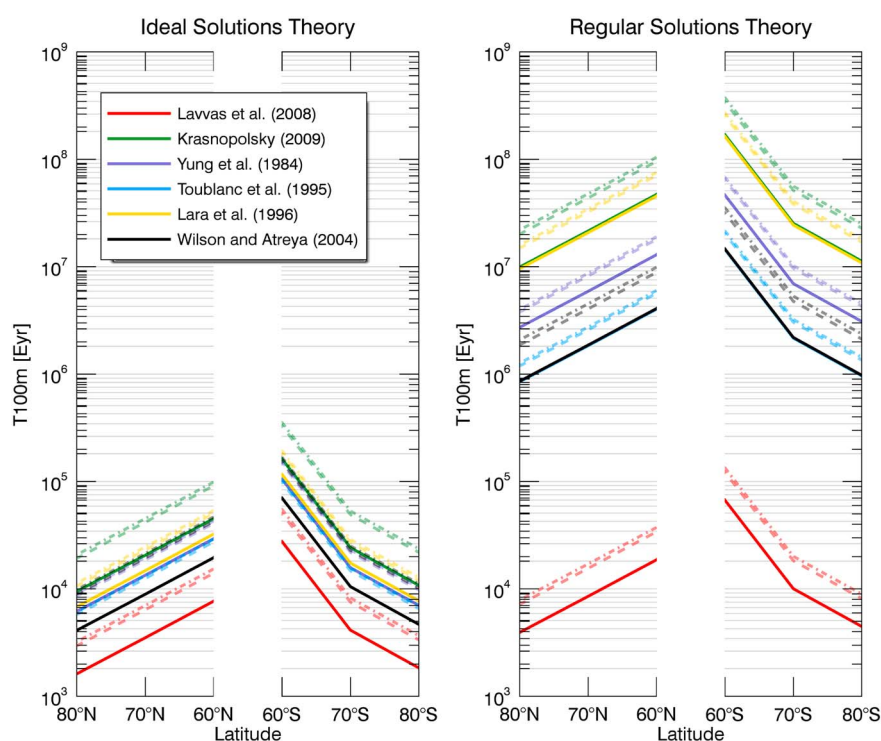
Figure 8. Same as Figure 7 but for the timescales of formation (in Eyr) of 100 m deep depressions on Titan.
