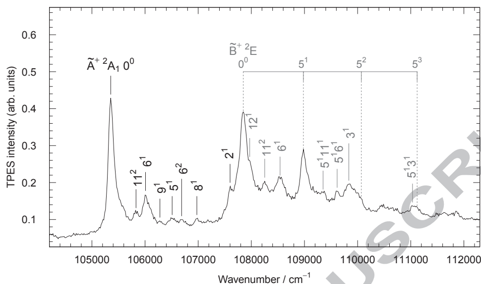
Figure 5: Threshold photoelectron spectrum of \text{CH}_3\text{C}_3\text{N} in the vicinity of the \tilde{\text{A}}^+ 2\text{A}_1 \leftarrow \tilde{\text{X}}^+ 1\text{A}_1 and \tilde{\text{B}}^+ 2\text{E} \leftarrow \tilde{\text{X}}^+ 1\text{A}_1 transitions with the assignments of the \tilde{\text{A}}^+ (in black) and \tilde{\text{B}}^+ (in gray) vibrational states.
