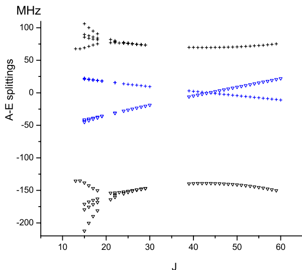
Fig. 1. A-E splitting of selected branches (R branches for K_a = 0; 1 in blue and 1;2 in black) for v_t = 1 . The x-axis represents the situation without perturbation. The A transitions ( \nabla signs) are twice as far as the E transitions (+ signs). For K_a = 0; 1 the A-E splitting changes sign at J = 44 (Ilyushin et al. 2009).
