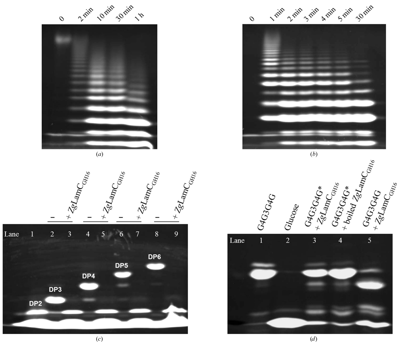
Figure 3 Mode of action and terminal products of ZgLamC GH16 . The hydrolysis of laminarin (a, c) and mixed-linked glucan (MLG) (b, d) by ZgLamC GH16 was monitored by fluorophore-assisted carbohydrate electrophoresis (FACE). (a) 0.5% (w/v) laminarin was hydrolyzed by 100 nM ZgLamC GH16 at 20°C. (b) 0.5% (w/v) MLG was hydrolyzed by 4.5 μM ZgLamC GH16 at 37°C. (c) Standard laminarin oligosaccharides are labelled from DP2 to DP6 (lanes 1, 2, 4, 6 and 8). 100 μg of the oligosaccharides from DP3 to DP6 at 0.1% were incubated with 4.5 μM ZgLamC GH16 at 37°C for 12 h (lanes 3, 5, 7 and 9). (d) The reaction mixtures contain 0.1% (w/v) of the tetrasaccharide G4G3G4G and 4.5 μM active (lane 3 and 5) or inactive (lane 4) ZgLamC GH16 in 100 mM phosphate–citrate pH 5.0 at 37°C for 30 min. An asterisk indicates that the G4G3G4G oligosaccharides were labelled before the enzymatic reaction, while the absence of an asterisk indicates that the oligosaccharides were labelled after the reaction.
