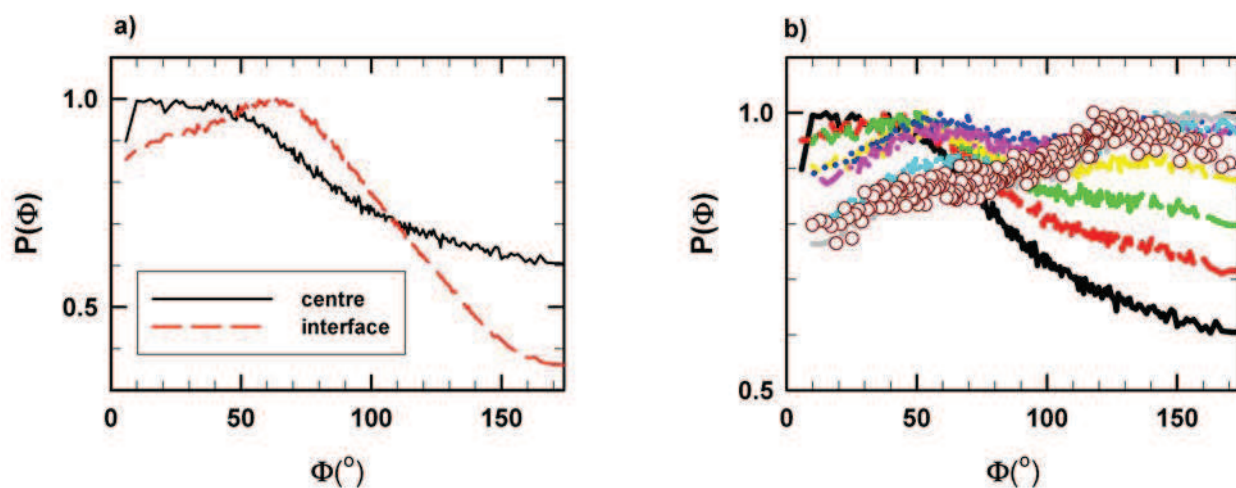
Fig. 4 a) Angular distribution between the dipolar moment of water molecules in the interfacial region and at the centre of the cavity and the outgoing normal vector to the silica surface. b) Angular distribution between the dipolar moment of water molecules at the centre of the cavity and the outgoing normal vector to the surface as a function of NaCl concentration. Color coding is the same as in Figure 3a. Empty symbols represent the results for c = 4.0 \text{ mol.L}^{-1} .
