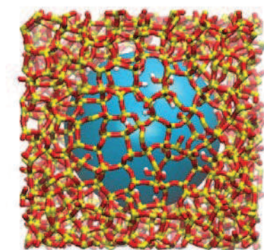
Fig. 1 Illustration of a spherical nanocavity (in cyan) carved in a silica cubic block. Red, yellow and white atoms correspond to oxygen, silicon and hydrogen atoms, respectively.
