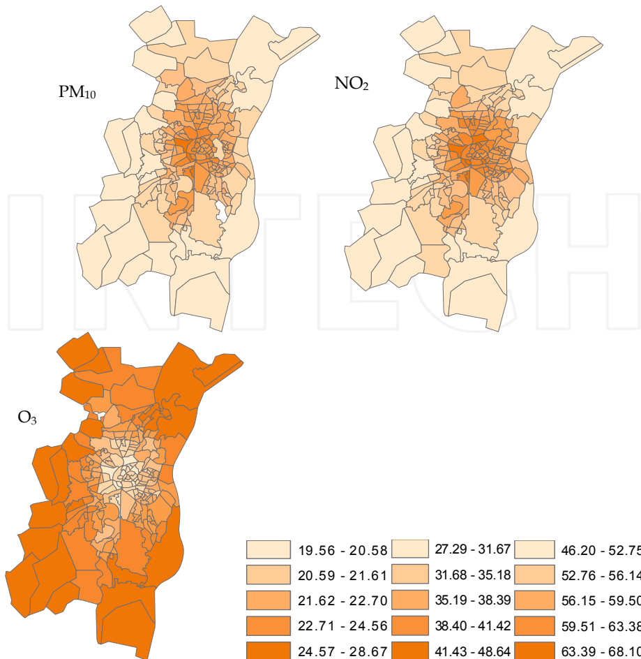
Fig. 3. Maps of ambient air pollutant concentrations ( \mu\text{g}/\text{m}^3 ) averaged by census block across the Strasbourg Metropolitan Area (2000-2005)
