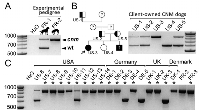
Figure 2. PTPLA mutation in the initial confirmation panel of CNM dogs. (A) Wild-type (wt = 610 bp) and PTPLA cnm (cnm = wt + 238 bp) alleles in a healthy carrier (FR-1) and an affected (FR-2) Labrador from the French experimental pedigree. (B) Segregation of the PTPLA cnm allele in a four-generation pedigree of a client-owned US proband female (arrow). (C) Genotypes of client-owned Labradors from several countries, diagnosed with CNM-related myopathies (asterisks; Table S1). US-6 is a champion known to have produced CNM pups; DE-5 is a control affected by a neuropathy and FR-2 was reloaded for size comparison. doi:10.1371/journal.pone.0046408.g002
