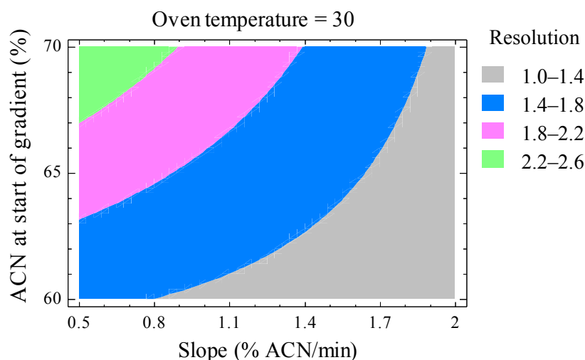
Figure 4. Chromatographic resolution between BMAA/DAB, optimized using a 2 3 factorial design. Since temperature did not influence the resolution significantly, it was set to 30 °C. A resolution of 1.5 corresponds approximately to the baseline resolution. ACN, acetonitrile.
