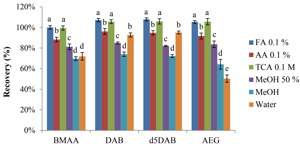
Figure 2. Recoveries of pure standards spiked at 30 ng/mL in different extraction solvents ( n = 3 , error bars represent standard deviations). Replicates with the same letter are not significantly different, while replicates with different letters are significantly different ( p < 0.05 ).
