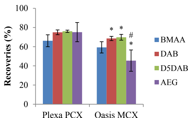
Figure 3. Recoveries of mixed solutions of standards spiked in TCA 0.1 M at a final concentration of 30 ng/mL. Comparison between 60 mg/3cc Plexa PCX and Oasis ® MCX cartridges ( n = 3 , error bars represent standard deviations). * p < 0.05 compared to recoveries with Plexa PCX. # p < 0.005 compared to D 5 DAB and DAB with Oasis ® MCX.
