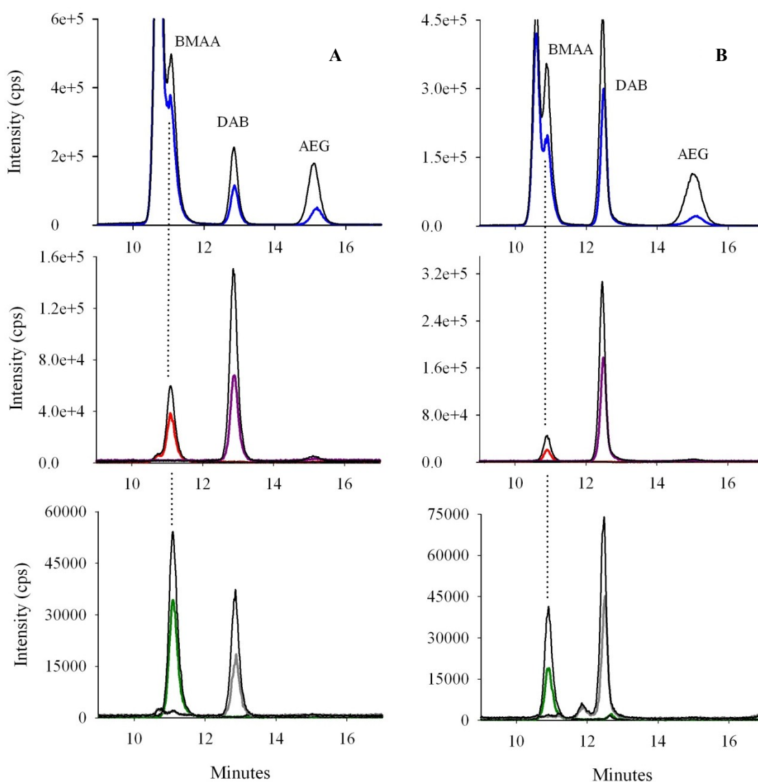
Figure 9. Chromatograms of spiked (dark line) and non-spiked, naturally-contaminated (A) oyster and (B) mussel samples after performing the extraction for the determination of total BMAA and isomers. Colored lines represent mass spectral transitions m/z 119 to m/z 102 (blue, top graphs), 88 (red) and 101 (purple) in the middle graphs and 76 (green) and 74 (grey) in the bottom graphs.
