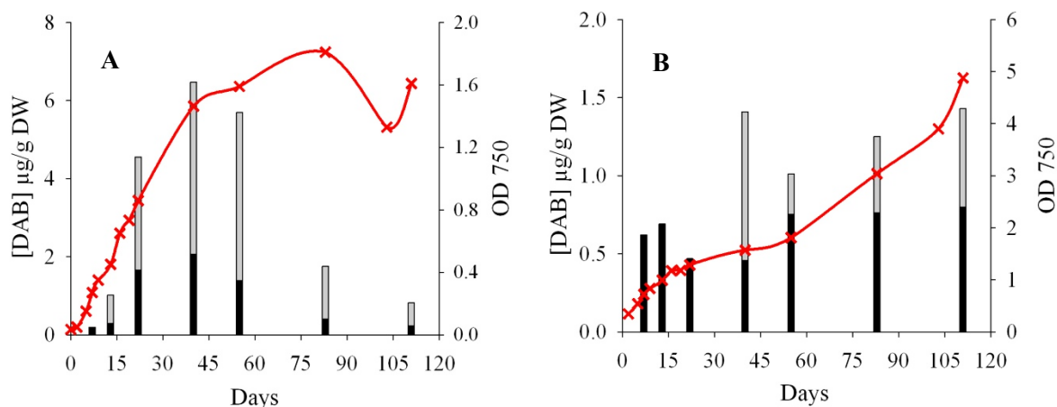
Figure 7. Growth curves (red line, cross symbols) and free (dark histograms) and bound (grey histograms) DAB concentration for (A) Nostoc CCMP 2511 and (B) Leptolyngbya PCC 73110.
