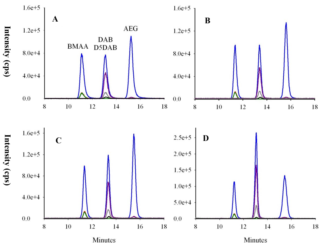
Figure 5. Chromatograms of BMAA, D 5 DAB and AEG spiked at 50 ng/mL into (A) standards; (B) cyanobacteria; (C) oyster and (D) mussel matrices after extraction of free analytes. Colored lines represent mass spectral transitions at m/z 119 to m/z 102 (blue), 88 (red), 76 (green), 101 (purple), 74 (grey) and m/z 124 to m/z 47 (dark).
