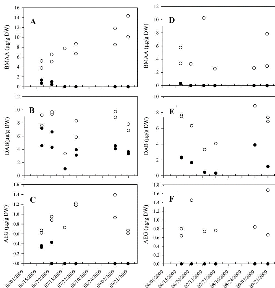
Figure 8. (A–C) BMAA, DAB and AEG concentrations in free (black circles) and total form (empty circles) in mussels collected in 2009 and (D–F) in oysters. Mollusks were sampled in two of the three areas where shellfish were cultured in the lagoon and analyzed for both areas when material was available.
