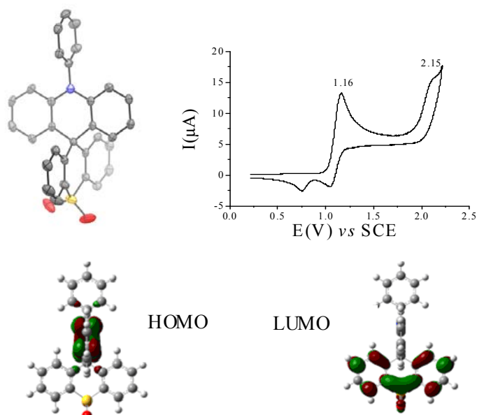
Fig 1. Top. ORTEP drawing (left, 50% ellipsoid probability) and cyclic voltammetry (100 \text{mV}\cdot\text{s}^{-1} ) in \text{CH}_2\text{Cl}_2/[\text{NBu}_4][\text{PF}_6] 0.2M (right) of SPA-TXO 2 . Bottom: Calculated nature of the highest occupied (HOMO) and lowest unoccupied (LUMO) orbitals of SPA-TXO 2 (isovalue 0.04)
