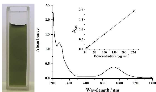
Figure 2. Picture of a dark-green solution of complex 3 in water ( c = 500\text{ }\mu\text{g}\cdot\text{mL}^{-1} ) (left) and UV-vis-NIR spectra of complex 3 in water ( c = 50\text{ }\mu\text{g}\cdot\text{mL}^{-1} ) (right) (insert: evolution of the absorbance at 940 nm as a function of the concentration).
