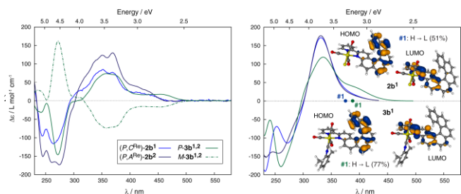
Figure 3. Left: experimental CD spectra of enantiopure complexes ( P,C^{Re} )-(+)- 2b^1 (light blue), ( P,A^{Re} )-(+)- 2b^2 (dark blue) and of ( M,CA^{Re} )-(-)- 3b^{1,2} (dotted green) and ( P,CA^{Re} )-(+)- 3b^{1,2} (plain green). Right: calculated CD spectra of ( P,C^{Re} )- 2b^1 , and ( P,A^{Re} )- 2b^2 and Boltzmann-averaged spectrum for P - 3b^{1,2} conformers. No spectral shift has been applied. View of HOMO and LUMO of 2b^1 and 3b^1 (0.04 au). First excitation energies indicated by dots on the abscissa.
