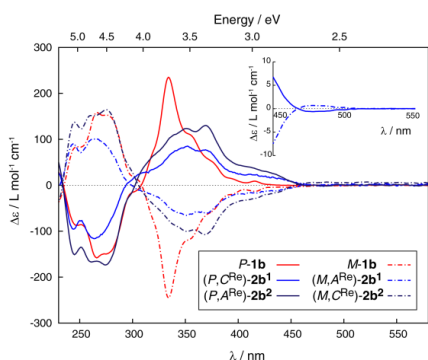
Figure 1. Experimental CD spectra of enantiopure M -(-) (dotted red) and P -(+)- 1b (plain red) and their corresponding enantiopure Re I complexes ( M , A Re )-(-)- 2b 1 and ( P , C Re )-(+)- 2b 1 (light blue) and ( M , C Re )-(-)- 2b 2 and ( P , A Re )-(+)- 2b 2 (dark blue). Inset: CD spectra of (-)- and (+)- 2b 1 between 450-550 nm.
