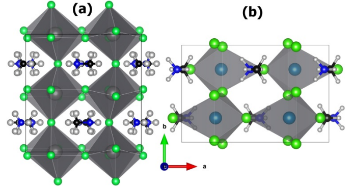
Fig. 3. Overview of the orthorhombic ( \text{Pnma} ) crystal structures of (a) \text{CH}_3\text{NH}_3\text{PbCl}_3 at low temperature (80 K) 24 and (b) \text{CH}_3\text{NH}_3\text{GeCl}_3 at room temperature (250 K) 22 . The unit cell of \text{CH}_3\text{NH}_3\text{PbCl}_3 is twice larger ( Z=8 ) than that of \text{CH}_3\text{NH}_3\text{GeCl}_3 ( Z=4 ) and related low temperature phases of \text{CH}_3\text{NH}_3\text{PbI}_3 26 and \text{CH}_3\text{NH}_3\text{PbBr}_3 , 25 and eight times larger than its room temperature disordered cubic phase ( \text{Pm}\bar{3}\text{m} , Z=1 ). 24,27 In addition to octahedral tilting, figure (b) highlights distortions that lead to pyramidal \text{GeCl}_3^- units.
