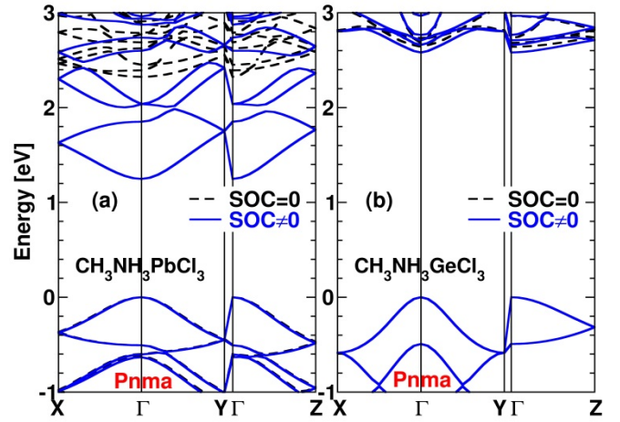
Fig. 7. Electronic band diagrams for the orthorhombic (Pnma) crystal structures shown Figure 3: (a) CH_3NH_3PbCl_3 and (b) CH_3NH_3GeCl_3 , calculated at the LDA level of theory without (black dashed lines) and with (blue straight lines) SOC.
