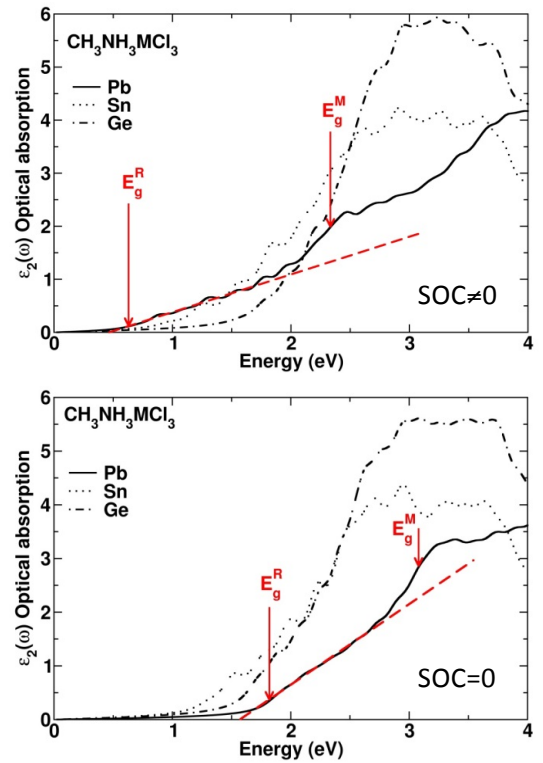
Fig. 5. Effect of metal substitution on the absorption spectra illustrated for \text{CH}_3\text{NH}_3\text{MCl}_3 ( \text{M}=\text{Pb}, \text{Sn}, \text{Ge} ): Absorption spectra calculated with (top) and without (bottom) SOC for the high temperature cubic structures ( \text{Pm}\bar{3}\text{m} ) of \text{CH}_3\text{NH}_3\text{MCl}_3 ( \text{M}=\text{Pb}, \text{Sn}, \text{Ge} ). Onsets of optical absorption at R and M are indicated for \text{CH}_3\text{NH}_3\text{PbCl}_3 .
