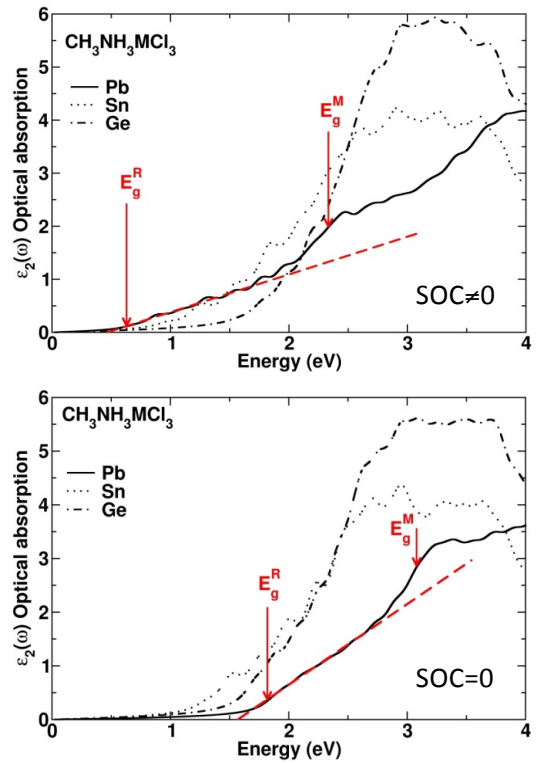
Fig. 5. Effect of metal substitution on the absorption spectra illustrated for \text{CH}_3\text{NH}_3\text{MCl}_3 ( \text{M}=\text{Pb} , \text{Sn} , \text{Ge} ): Absorption spectra calculated with (top) and without (bottom) SOC for the high temperature cubic structures ( \text{Pm}\bar{3}\text{m} ) of \text{CH}_3\text{NH}_3\text{MCl}_3 ( \text{M}=\text{Pb} , \text{Sn} , \text{Ge} ). Onsets of optical absorption at R and M are indicated for \text{CH}_3\text{NH}_3\text{PbCl}_3 .
