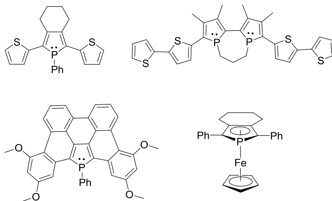
Figure 1: Example of phosphole based \pi -conjugated systems
