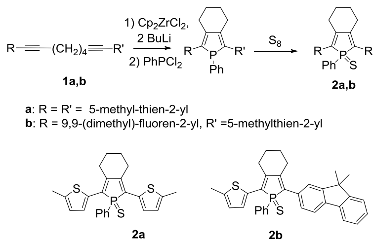
Scheme 1. Synthetic routes to phosphole-based dopants
