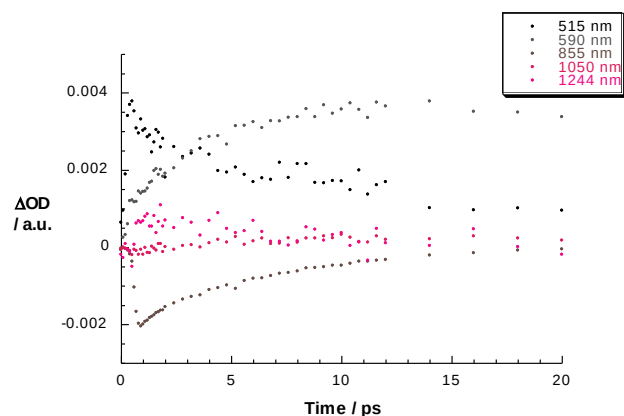
Figure 6. Upper part – differential absorption spectra (visible and near-infrared) obtained upon femtosecond flash photolysis (778 nm) of 2 in benzonitrile with several time delays between 0 and 10 ps at room temperature – time development from black to red to blue to yellow and yellow. Lower part – time-absorption profiles of the spectra shown in the upper part at 515, 590, 855, 1050, and 1244 nm monitoring the competition between formation of the singlet excited state and charge separation as well as charge recombination.
