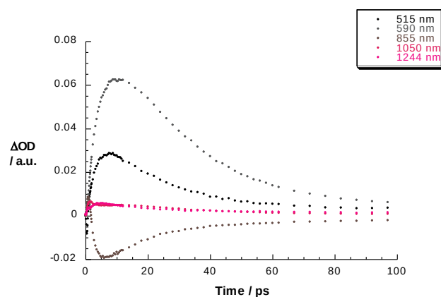
Figure 4. Upper part – differential absorption spectra (visible and near-infrared) obtained upon femtosecond flash photolysis (387 nm) of 2 in benzonitrile with several time delays between 0 and 100 ps at room temperature – time development from black to red to blue to yellow and yellow. Lower part – time-absorption profiles of the spectra shown in the upper part at 515, 590, 855, 1050, and 1244 nm monitoring the charge separation and charge recombination.
