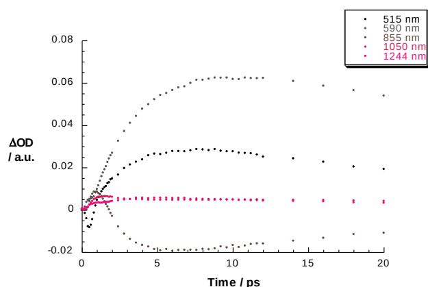
Figure 3. Upper part – differential absorption spectra (visible and near-infrared) obtained upon femtosecond flash photolysis (387 nm) of 2 in benzonitrile with several time delays between 0 and 10 ps at room temperature – time development from black to red to blue to orange and yellow. Lower part – time-absorption profiles of the spectra shown in the upper part at 515, 590, 855, 1050, and 1244 nm monitoring the competition between formation of the singlet excited state and charge separation as well as charge recombination.
