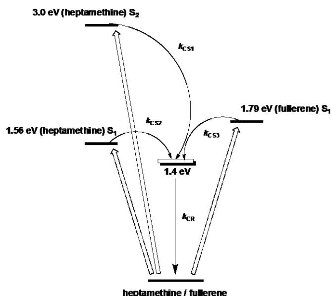
Figure 7. Energy diagram illustrating the different excitation, charge separation ( k_{CS1} , k_{CS2} , k_{CS3} – see for Table 1 for details), and charge recombination ( k_{CR} ) pathways in 2 and 3.
