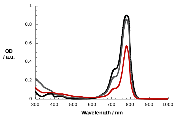
Figure 1. Absorption spectra of 1 (black spectrum), 2 (grey spectrum), and 3 (red spectrum) – 5.0 \times 10^{-6} M – recorded in dichloromethane
