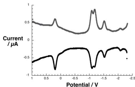
Figure 2. Upper part – cyclic voltammogram of 2 recorded in deaerated dichloromethane versus the ferrocene/ferricenium couple – TBAPF 6 was employed as supporting electrolyte. Lower part – corresponding differential pulse voltammogram.
