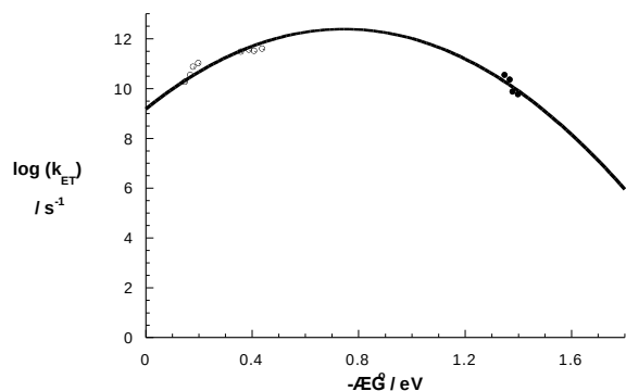
Figure 5. Driving force ( -\Delta G^0 ) dependence of the rate constant for charge separation (open circles) and charge recombination (full circles).
