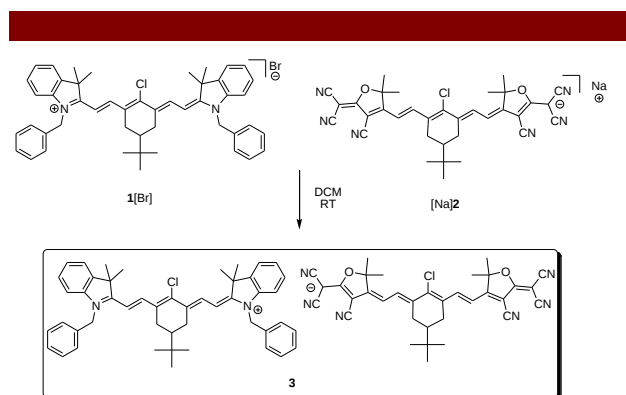
Figure 1. Synthesis and structure of the new dye 3 .
