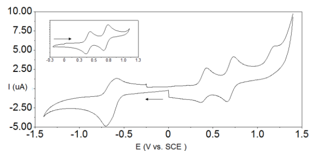
Figure 3. CV trace obtained for 3 (CH 2 Cl 2 , 0.2 M Bu 4 NPF 6 , \nu = 100 \text{ mV.s}^{-1} ). Inset shows the reversibility of the first two oxidation processes.
