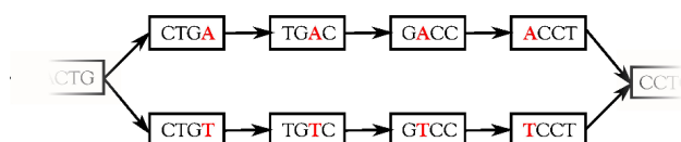
Figure 2. Toy example of a Bubble in the de Bruijn Graph ( k=4 ). Bubble generated by a single nucleotide polymorphism. The two polymorphic sequences are ...CTGACCT... and ...CTGTCCT....
