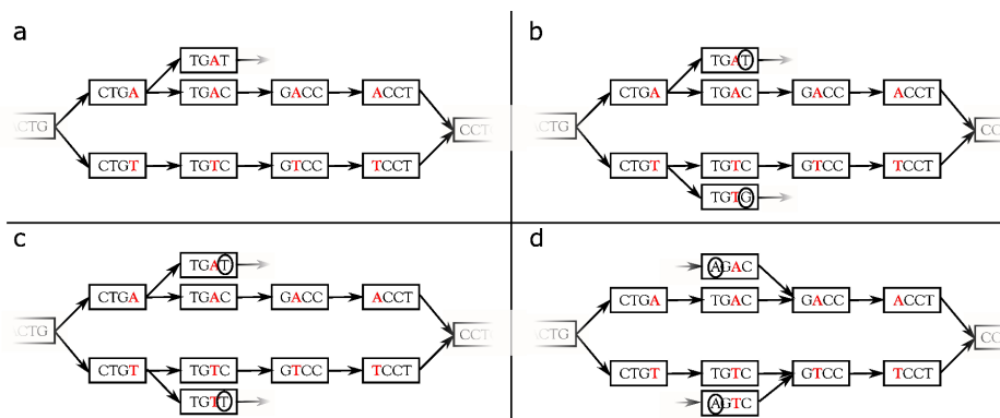
Figure 3. Examples of non symmetrically branching bubbles ( a and b ) and symmetrically branching bubbles ( c and d ). Path divergences in bubbles a and b create branching bubbles, but the branching is not symmetric. Divergence is only present in one path ( a ) or in both paths but with distinct (circled) characters ( b ). Path divergences in bubbles c and d create symmetrically branching bubbles. Both paths of these bubbles can be right extended ( c ) or left extended ( d ) with the same two (circled) characters. With option -b 0 (default), none of these bubbles would be considered as a SNP, with option -b 1 bubbles a and b would have been considered as SNP while with option -b 2 all of them would have been output.
