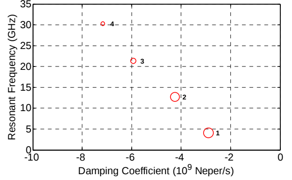
Fig. 2 Resonant poles in the complex plane, extracted from the field backscattered by a dipole antenna with |R|/|\alpha| weighting.
