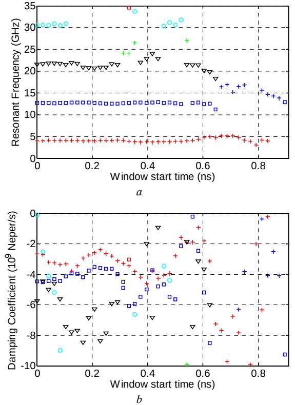
Fig. 3 WMT applied on the electric far field backscattered by a dipole antenna
