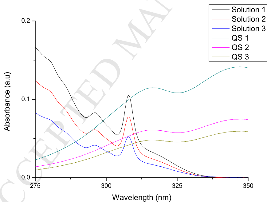
S 12 Quantum yield measurements: Absorption of solutions of 4-5Pm-SBF in cyclohexane and quinone sulfate (QS) in H 2 SO 4 1N
