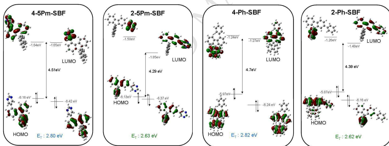
Figure 3. Calculated frontier molecular orbitals by DFT of 4-5Pm-SBF ; 4-Ph-SBF ; 2-5Pm-SBF and 2-Ph-SBF , after geometry optimization at the B3LYP/6-311G+(d,p) level of theory, shown with an isovalue of 0.04 .
